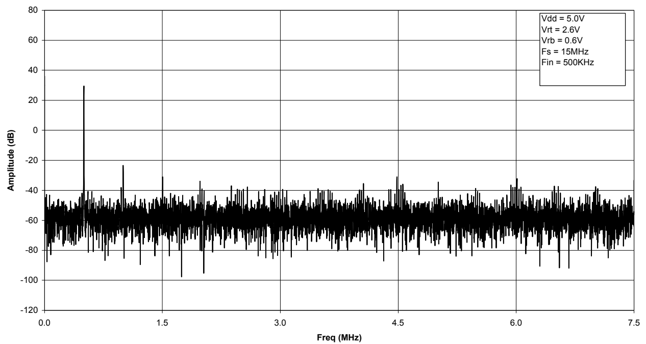
Graph 10. FFT Plot
