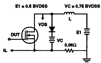
FIGURE 2. CLAMPED INDUCTIVE SWITCHING, ILM
