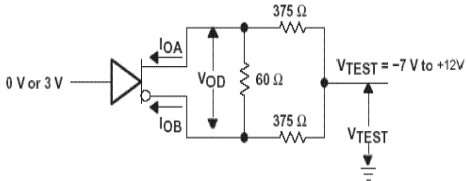
Figure 2. Driver Test Circuit, VOD With Common-Mode Loading
