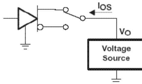
Figure 7. Driver Short-Circuit Test Configuration
