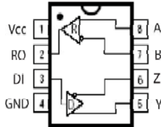
8-Pin PDIP/nSOIC
