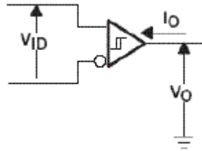
Figure 8. Receiver Parameter Definitions
