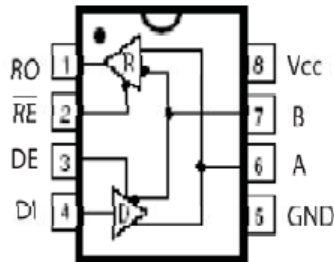
8-Pin PDIP/nSOIC
