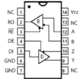
14-Pin PDIP/nSOIC
