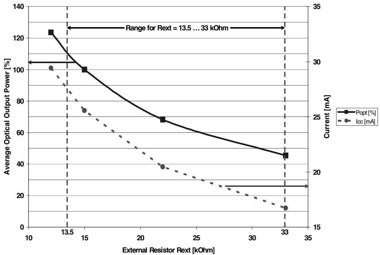
Figure 1. Typical Dependency of Average Optical Output Power P_{opt} and Supply Current versus External Resistor R_{ext} (22.5 Mbit MOST Data, V_{CC} = 5.0 V, T_A = 25 °C)
