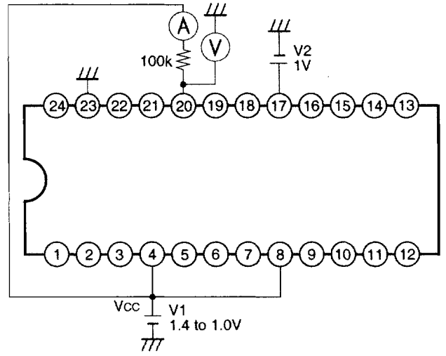
Measurement circuit 6
