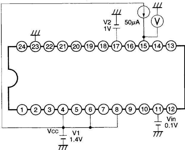
Measurement circuit 9
