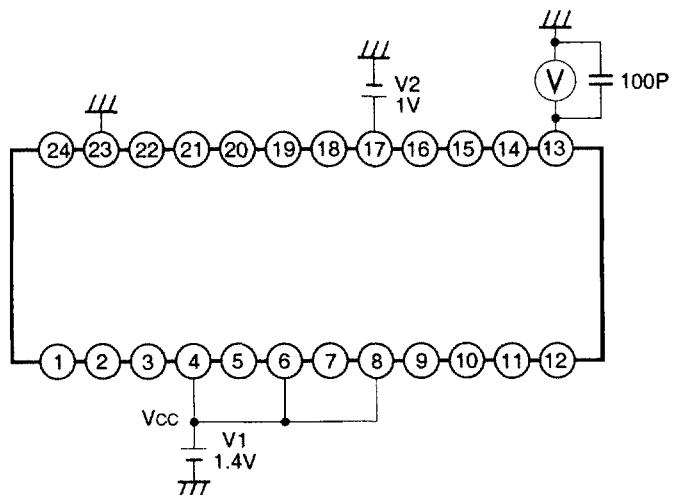
Measurement circuit 10
