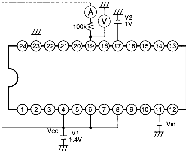
Measurement circuit 3
