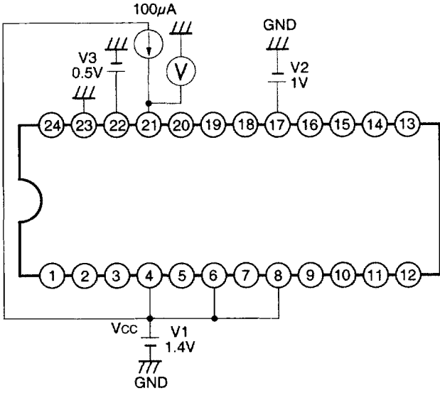
Measurement circuit 5
