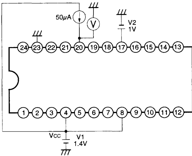
Measurement circuit 7
