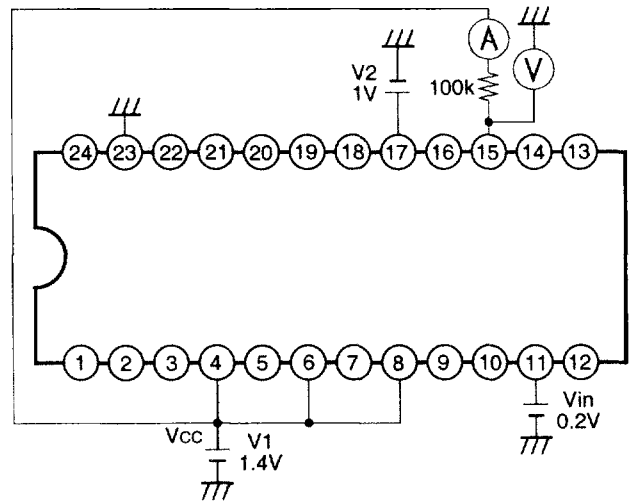
Measurement circuit 8
