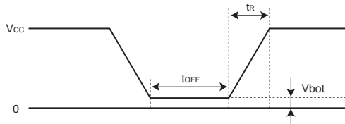
Fig.64 Rise waveform
