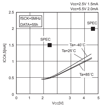
Fig.15 Consumption current at READ operation ICC_{4,5}(READ, WRSR, f_{SCK}=5MHz)
