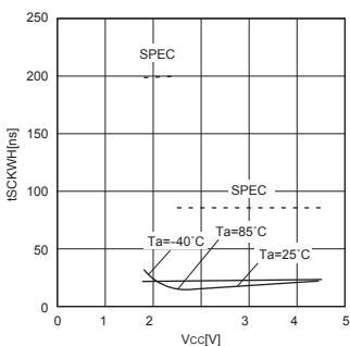
Fig.18 t_{SCKWH} high time t_{SCKWH}
