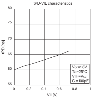
Fig.55 VIL dependency of data output delay time
