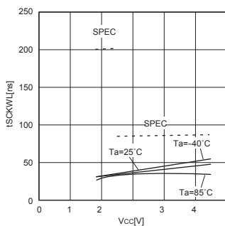
Fig.19 t_{SCKWL} low time t_{SCKWL}
