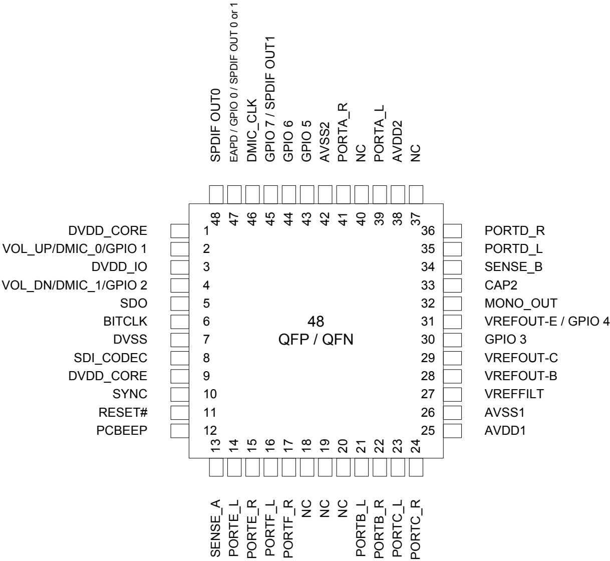
Figure 12. Pin Assignment
