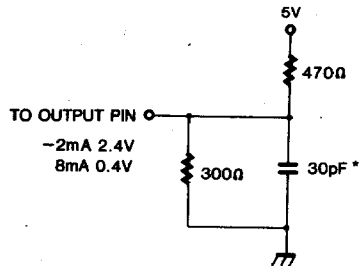
Figure 1. Output Load
