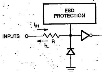
Figure 1. Input Structure
