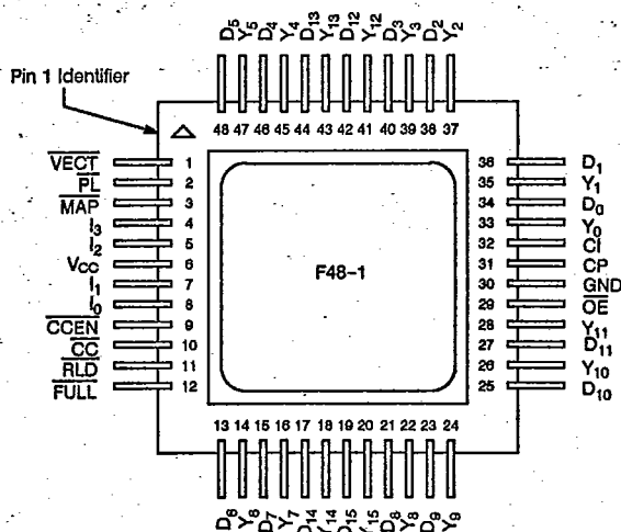
FLATPACK TOP VIEW
