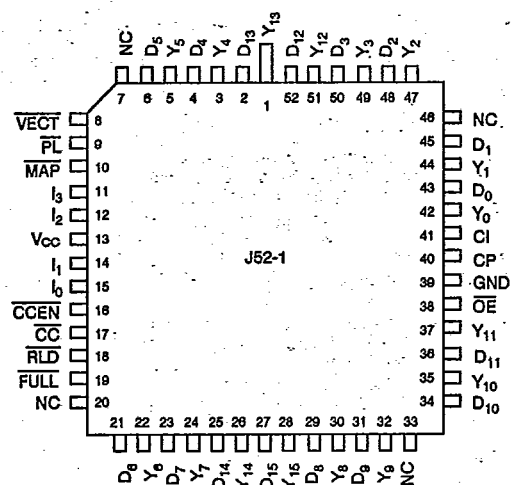
PLCC TOP VIEW
