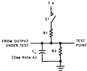
LOAD CIRCUIT
