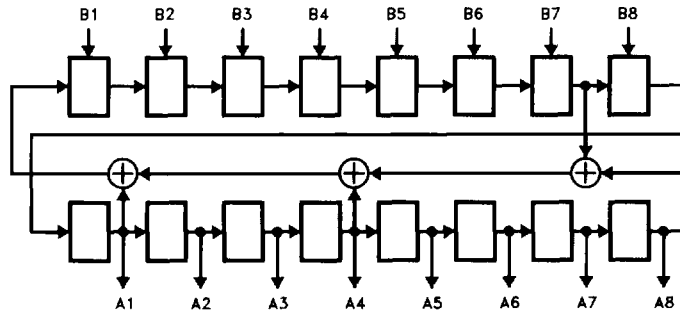
FIGURE 10. 16-BIT PRPG CONFIGURATION (B TO A MODE)
