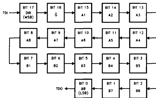
FIGURE 3. BOUNDARY SCAN REGISTER ORDER OF SCAN (A TO B MODE)
