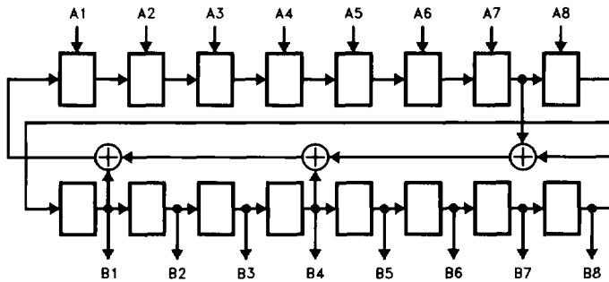
FIGURE 9. 16-BIT PRPG CONFIGURATION (A TO B MODE)
