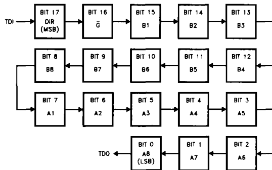
FIGURE 4. BOUNDARY SCAN REGISTER ORDER OF SCAN (B TO A MODE)
