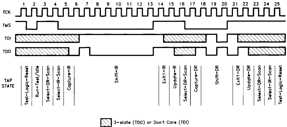
FIGURE 13. TIMING EXAMPLE
