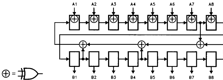
FIGURE 7. 16-BIT PSA CONFIGURATION (A TO B MODE)
