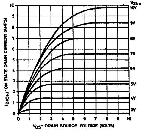
Fig. 2 Typical saturation characteristics
