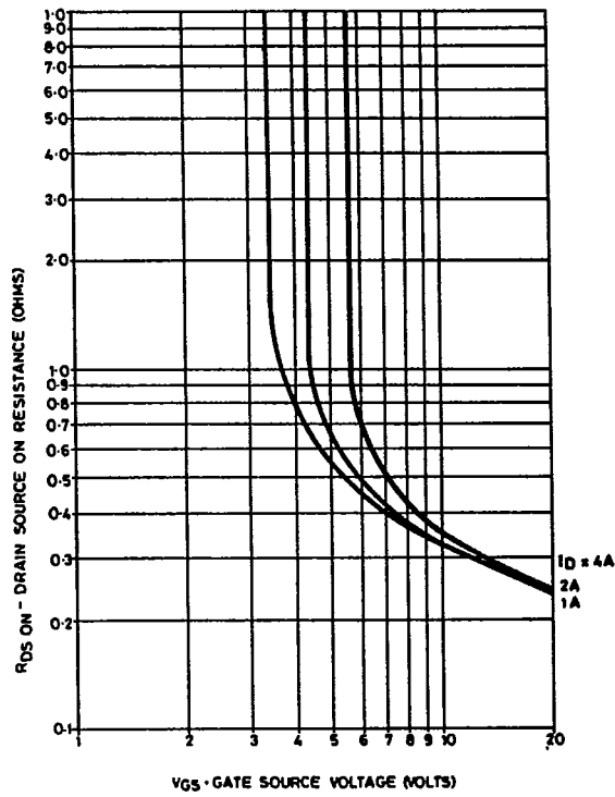
Fig. 5 Typical on-resistance v gate-source voltage
