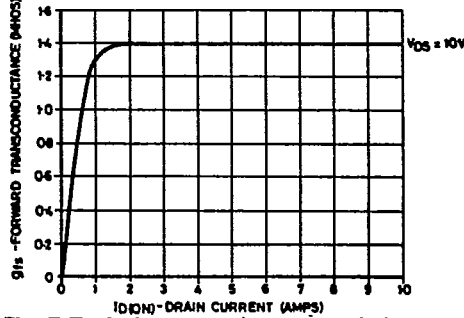
Fig. 7 Typical transconductance v drain current
