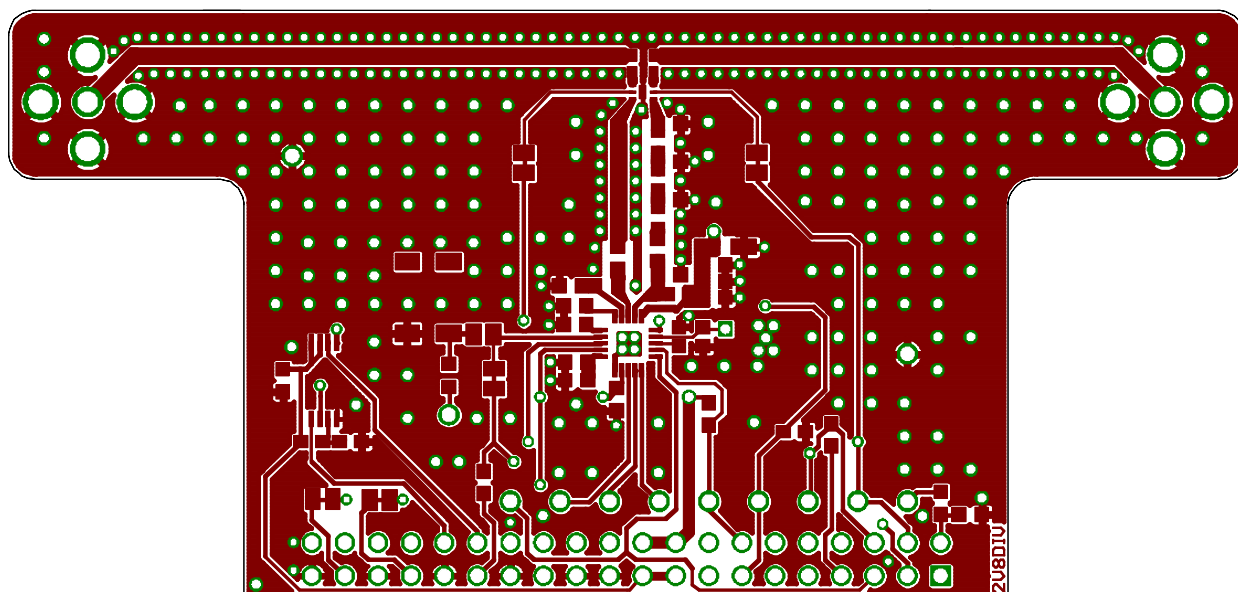
Figure 41. Antenna Diversity Reference Design - Top
