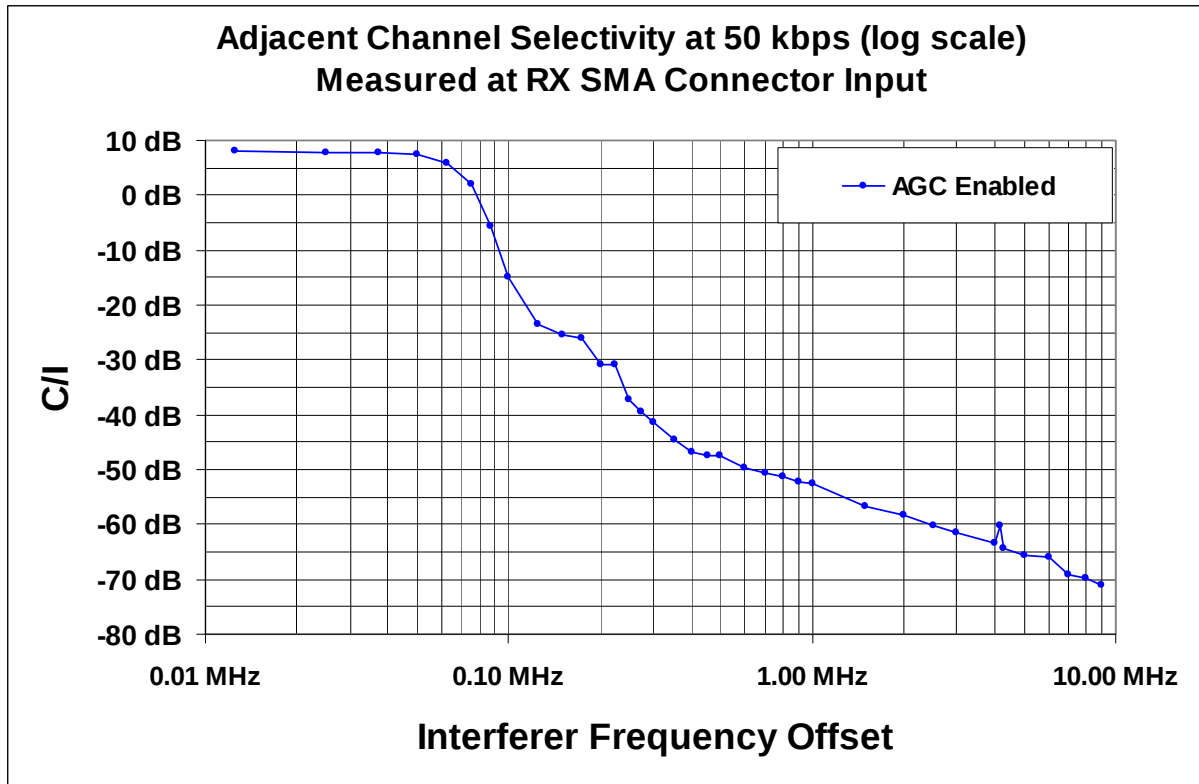
Figure 45. Receiver Selectivity
