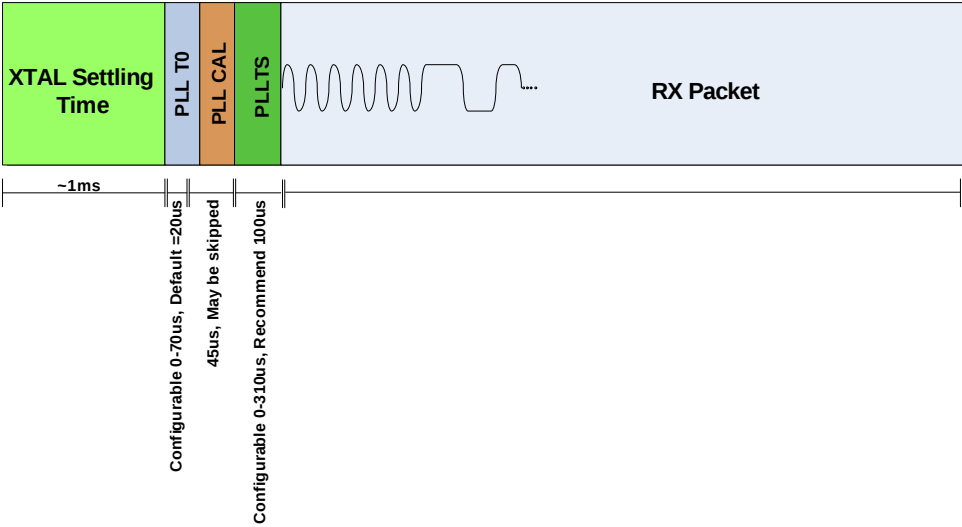
Figure 8. RX Timing
