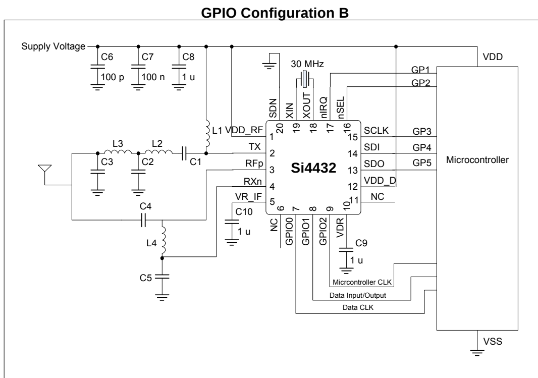
Figure 30. GPIO Usage Examples
