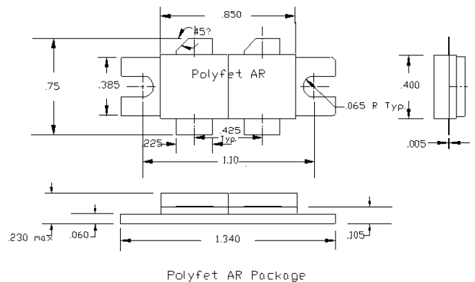
PACKAGE DIMENSIONS IN INCHES
