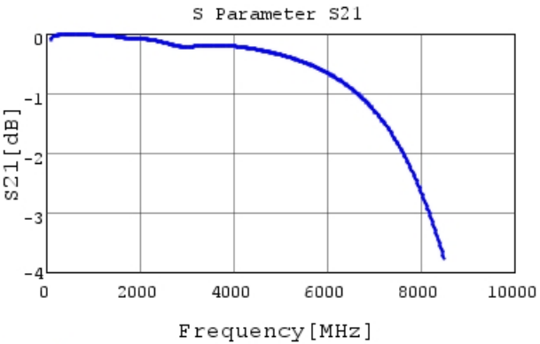
GCM1885C1H101JA16 S21 DCOV, 25degC
