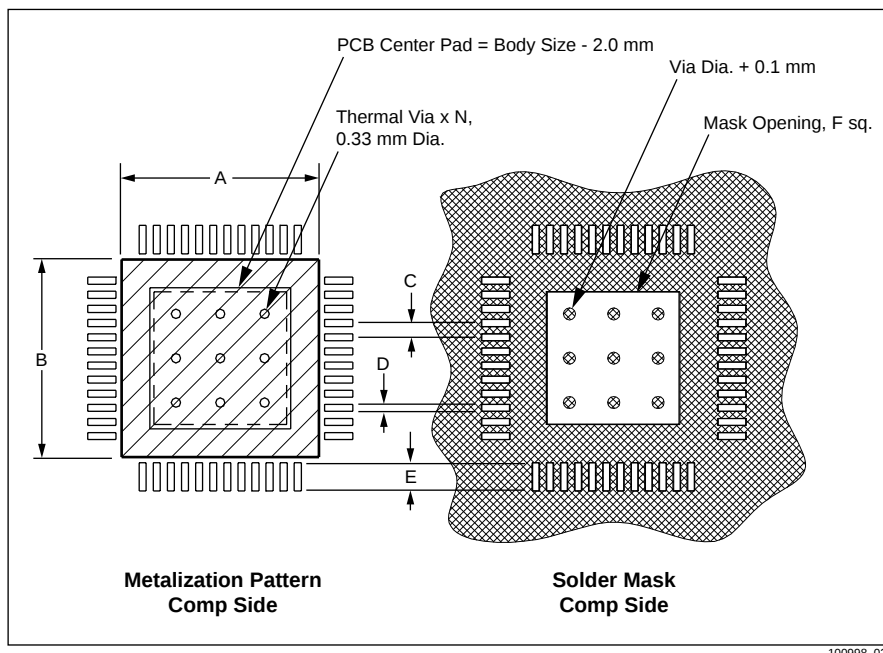
Figure B-2. Package and PCB Land Configuration
