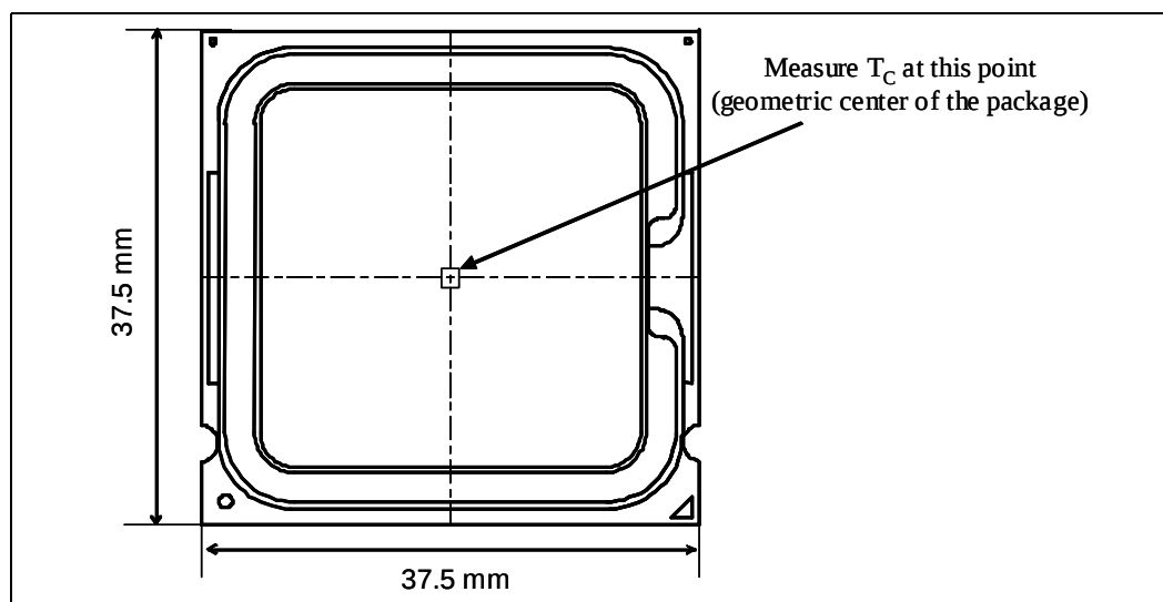
Figure 5-2. Case Temperature ( T_C ) Measurement Location
