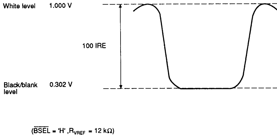
Figure 16 HD153109CP and HD153109MA VIDEO Output Waveform (In case of \overline{\text{SYNC}} signal non-composite)
