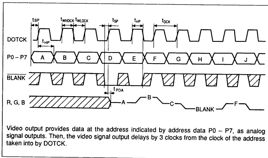
Figure 9 Video Output
