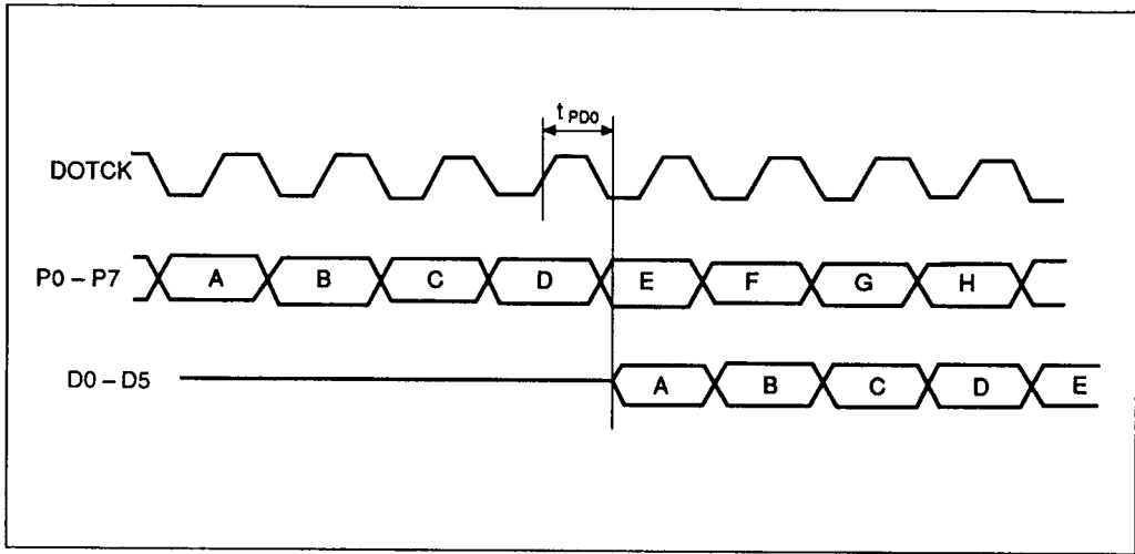
Figure 12 Digital Output
