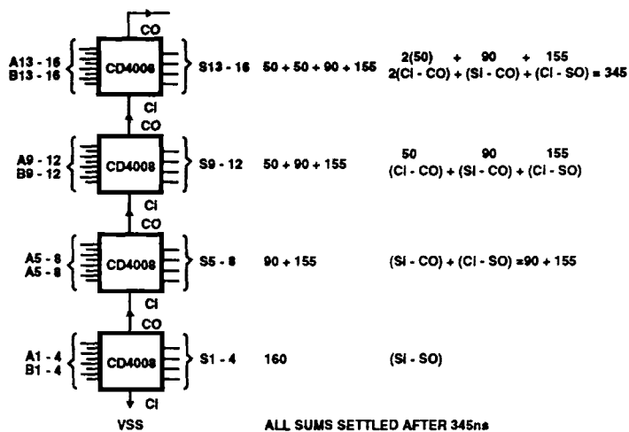
FIGURE 1. PROPAGATION DELAY FOR A 16 BIT ADDER (10V OPERATION)
