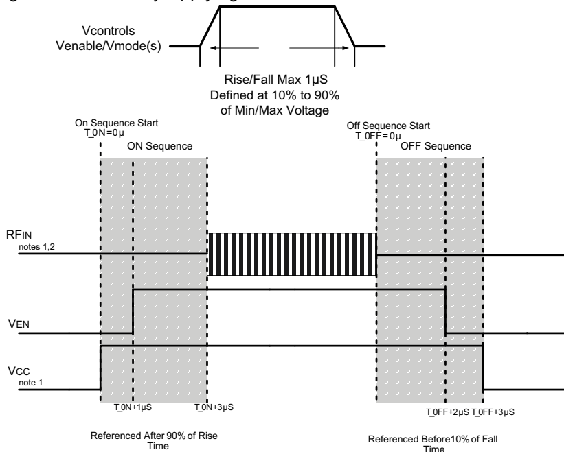
Figure 3: Minimum Recommended ON/OFF Timing Sequence
