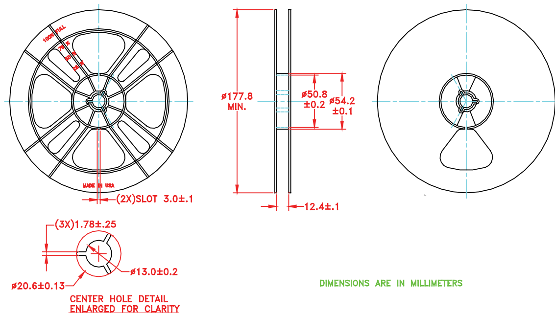
Figure 8: Carrier Tape
