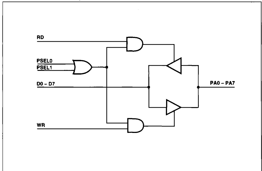
Figure 34. Port A In Peripheral I/O Mode
