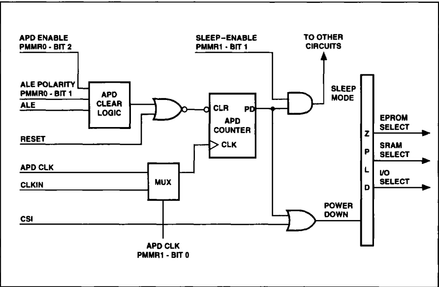
Figure 37. Power Management Unit
