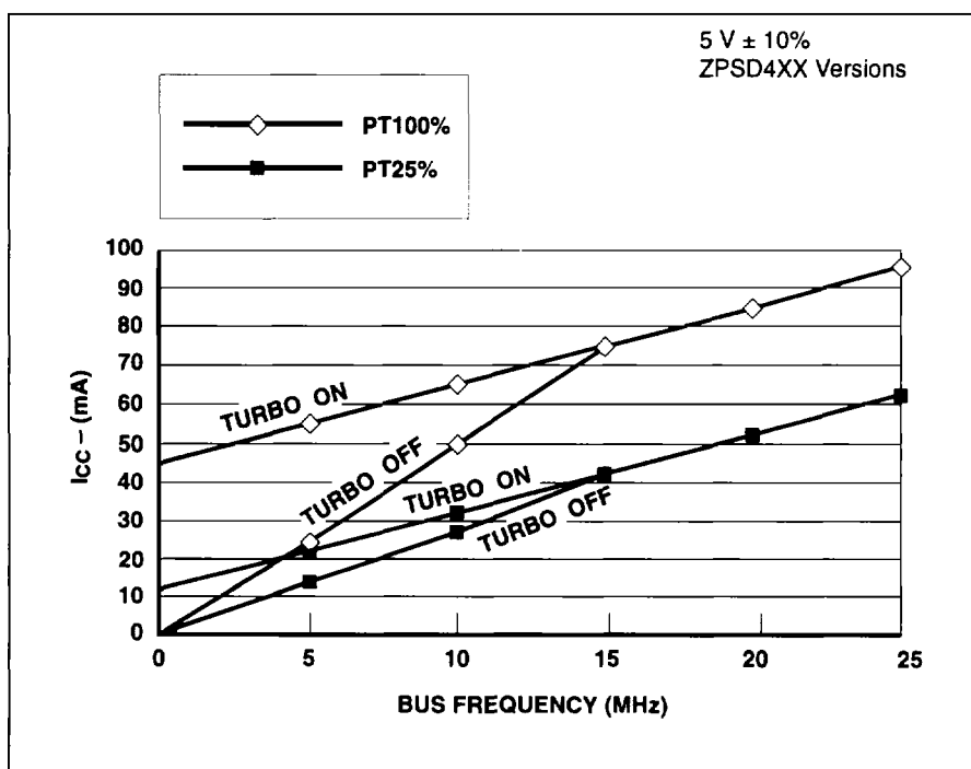
Figure 38a. ZPLD I_{CC} /Frequency Consumption
