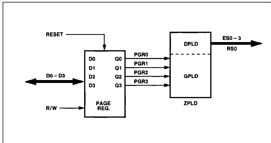
Figure 36. Page Register
