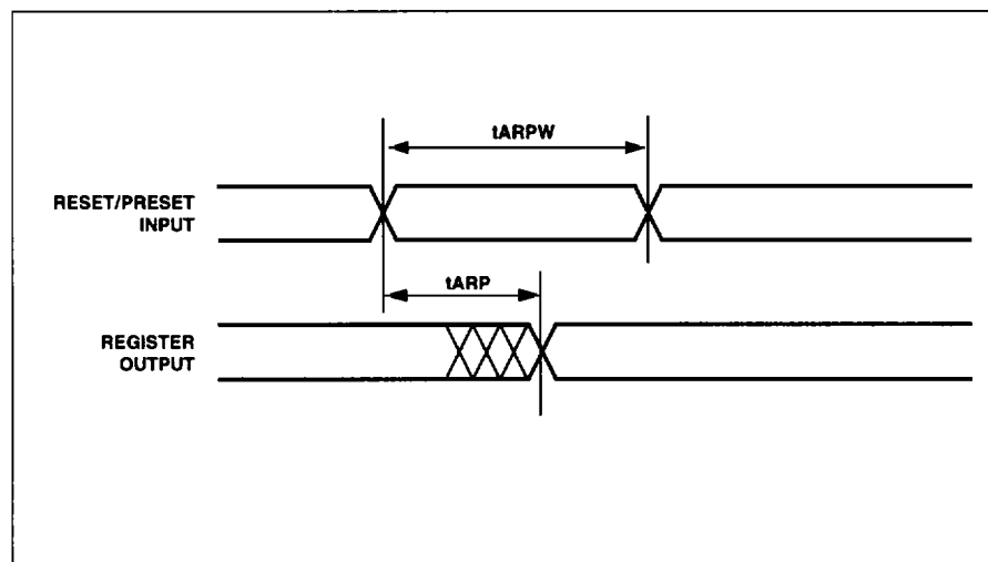
Figure 47. Asynchronous Reset/Preset
