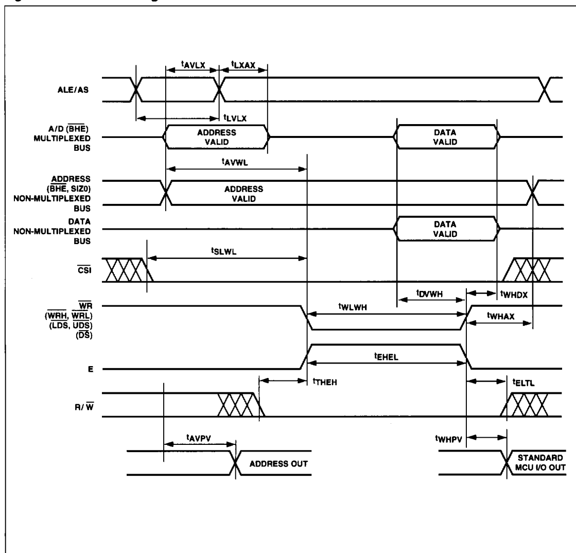
Figure 40. Write Timing
