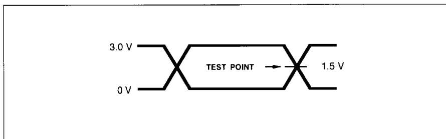
Figure 50. AC Testing Input/Output Waveform
