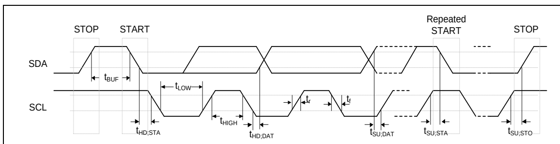
Figure 6.15-2 I²C Bus Timing
