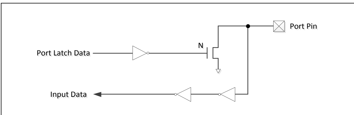
Figure 6.6-3 Open-Drain Output
