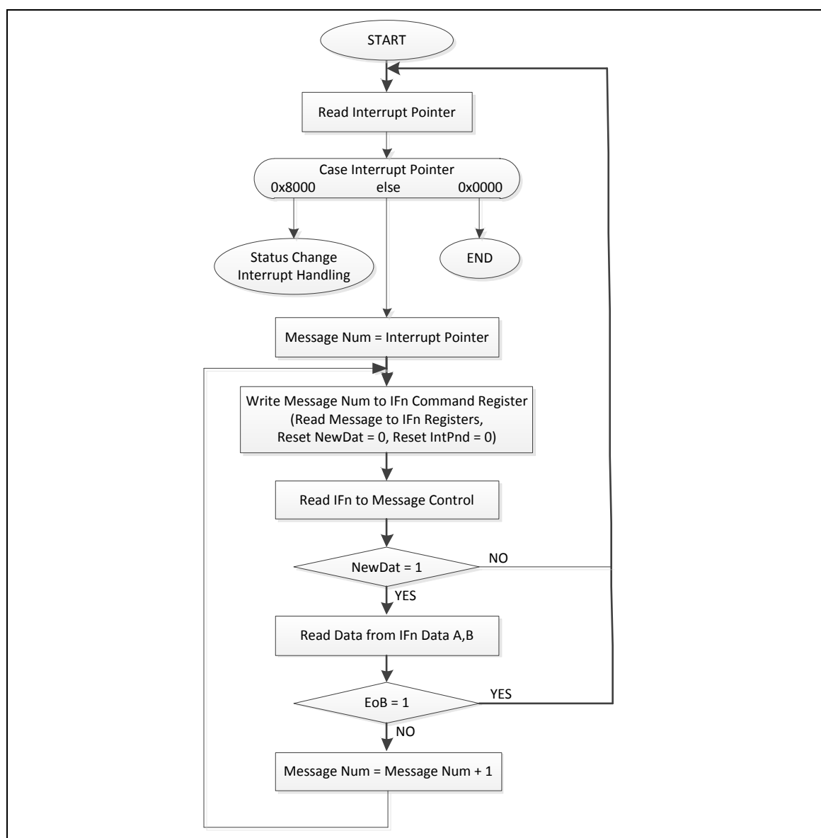
Figure 6.20-6 Application Software Handling of a FIFO Buffer
