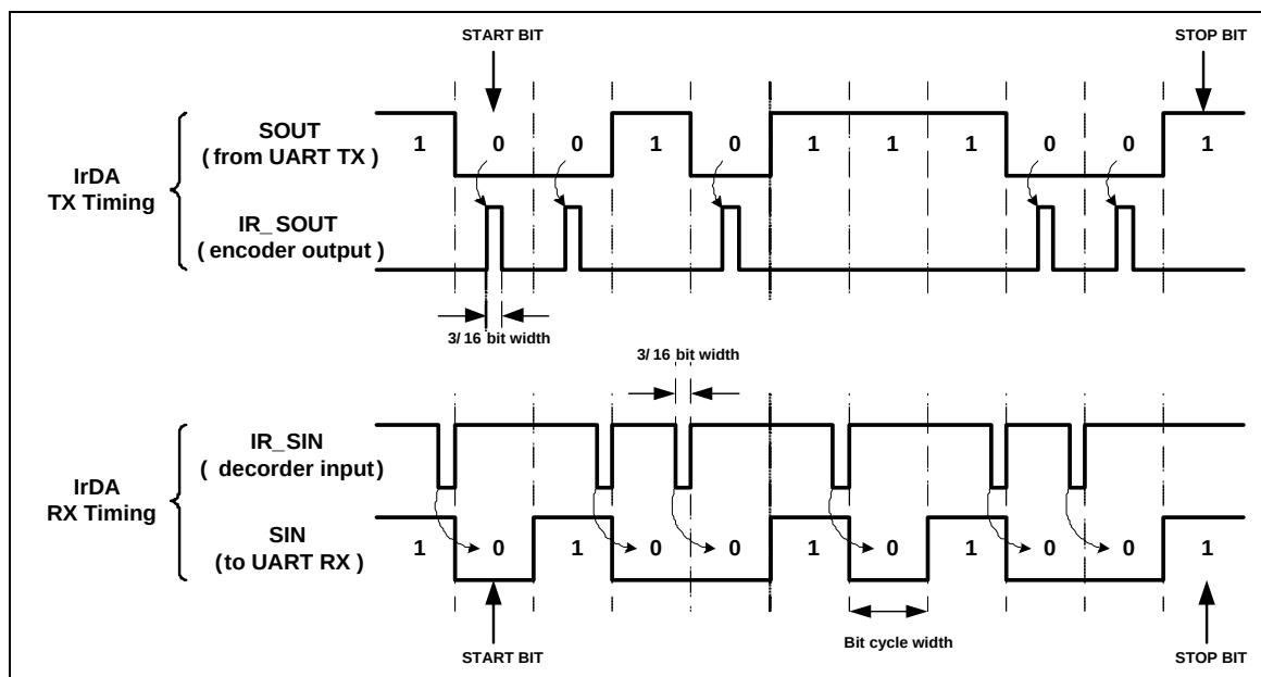
Figure 6.13-13 IrDA TX/RX Timing Diagram
