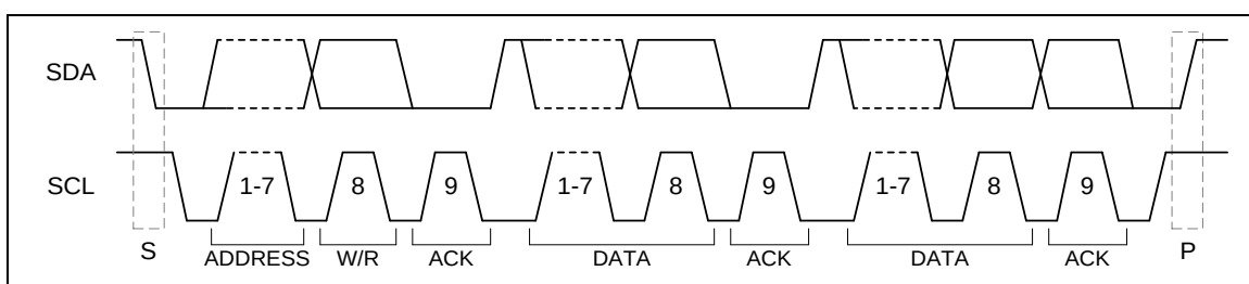
Figure 6.15-3 I²C Protocol
