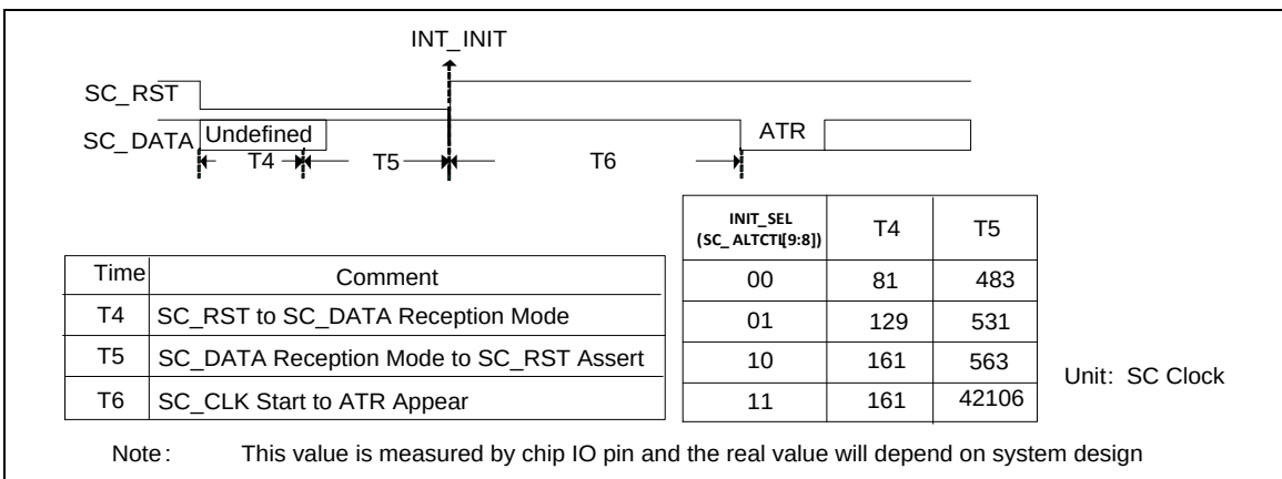
Figure 6.14-5 SC Warm Reset Sequence
