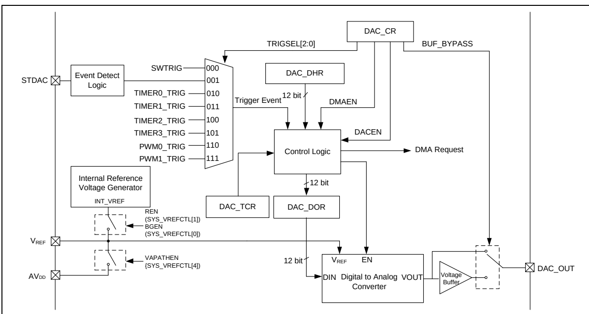
Figure 6.24-1 Digital-to-Analog Converter Block Diagram
