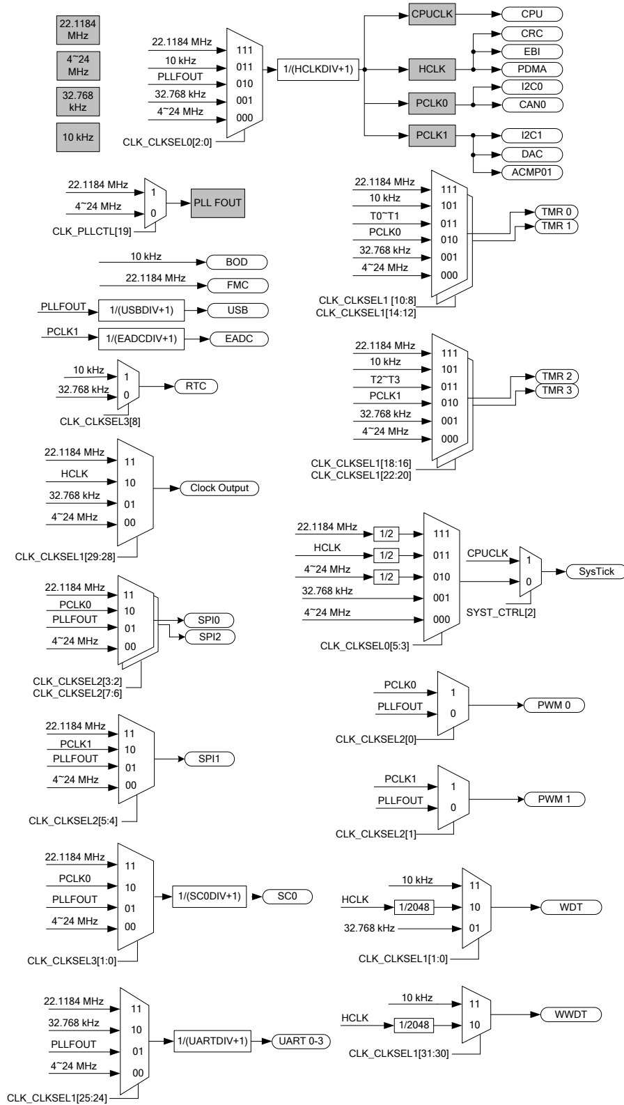
Figure 6.3-1 Clock Generator Global View Diagram
