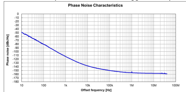
Phase Jitter (12 kHz to 20 MHz): 30 fs Typ.
