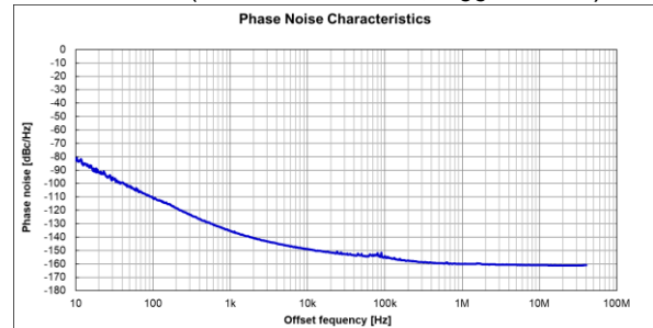
Phase Jitter (12 kHz to 20 MHz): 60 fs Typ.
