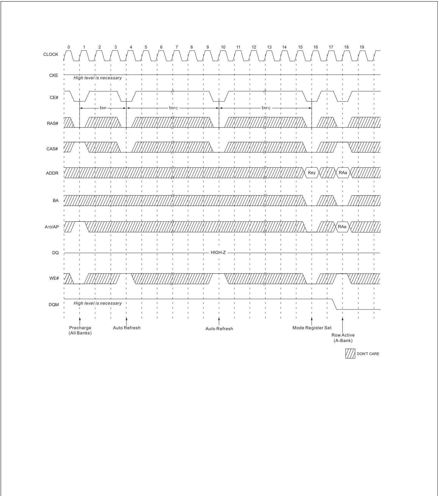
FIGURE 3 – POWER UP SEQUENCE
