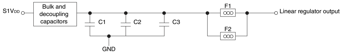
Figure 85. S1V DD power supply filter circuit
