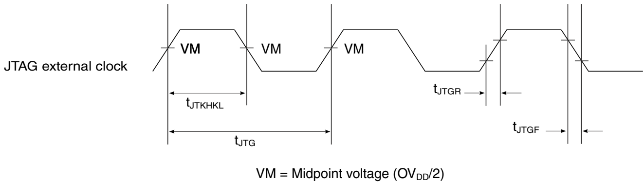
Figure 67. JTAG clock input timing diagram
