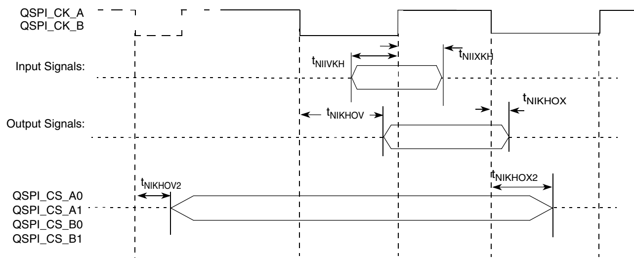
Figure 56. QuadSPI AC timing — SDR mode
