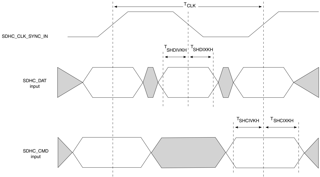
Figure 63. eSDHC DDR50/eMMC DDR mode input AC timing diagram
