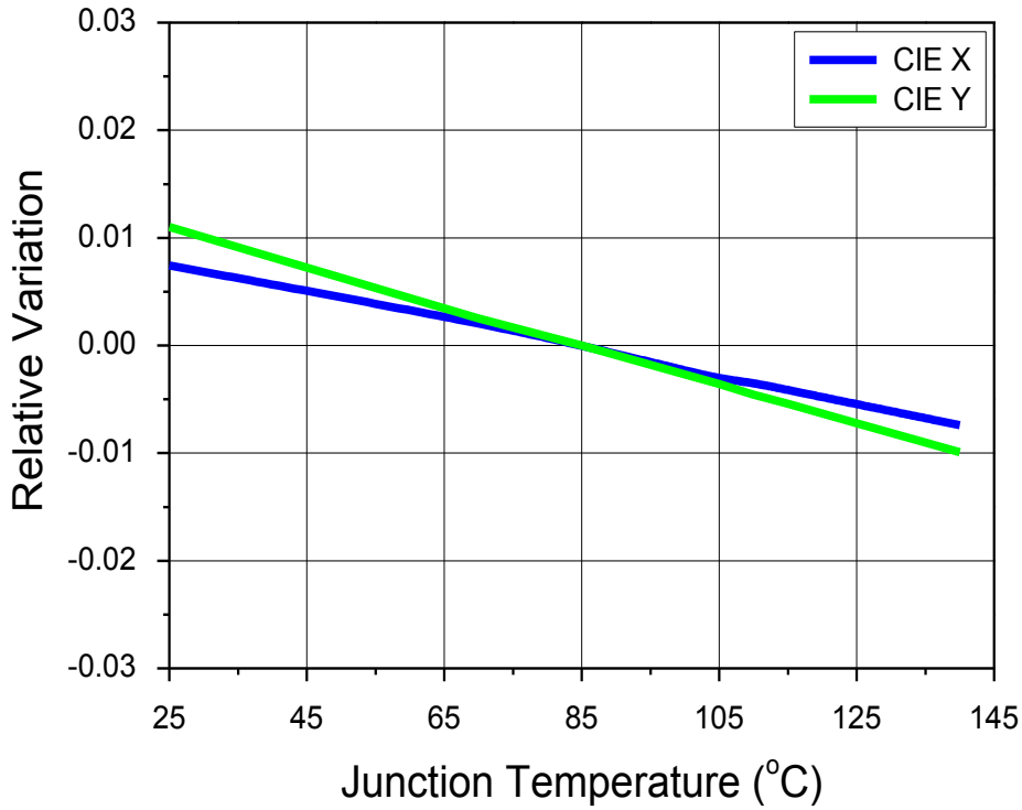
Fig 13. Junction Temperature vs. CIE x,y Shift, I_f=0.24A (CRI80, Cool White)
