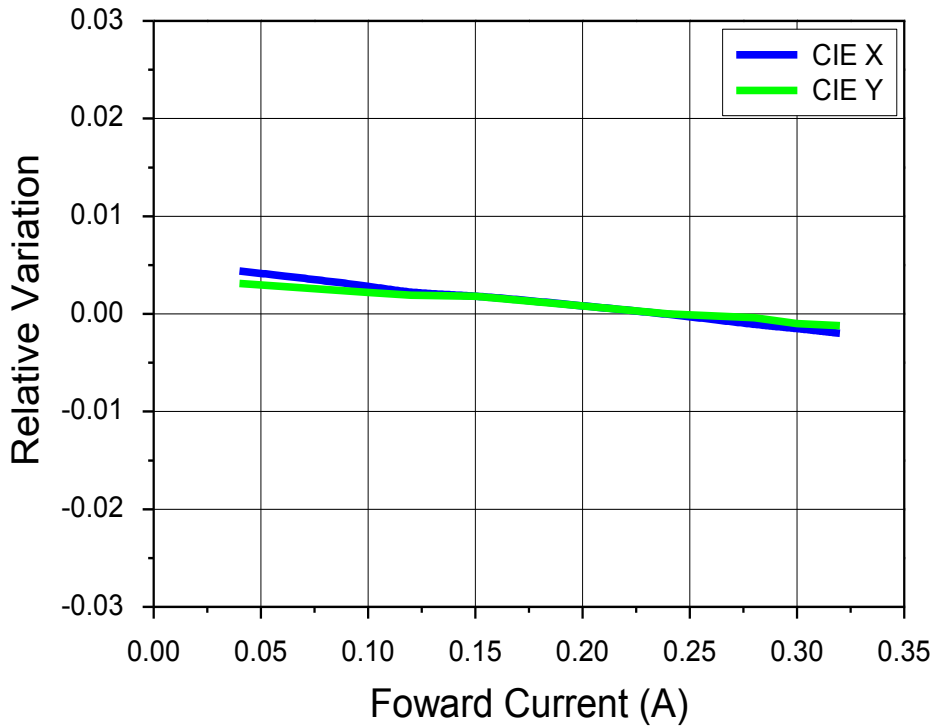
Fig 8. Forward Current vs. CIE x,y Shift (CRI80, Warm White)
