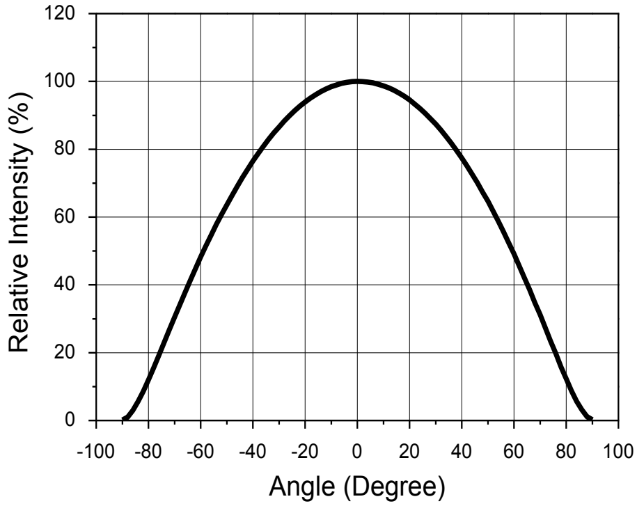
Fig 3. Radiant Pattern, I_F = 0.24A
