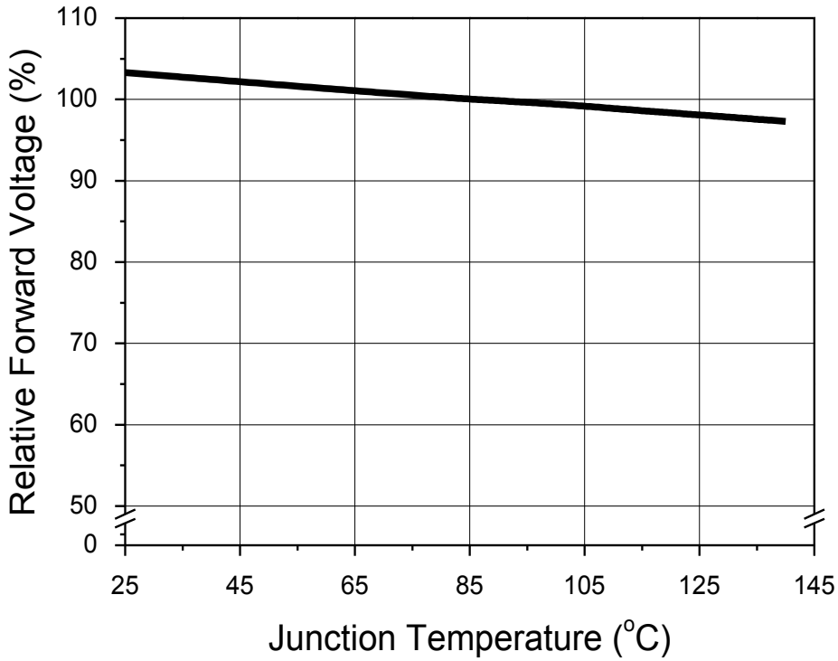
Fig 11. Junction Temperature vs. Forward Voltage, I_F=0.24A
