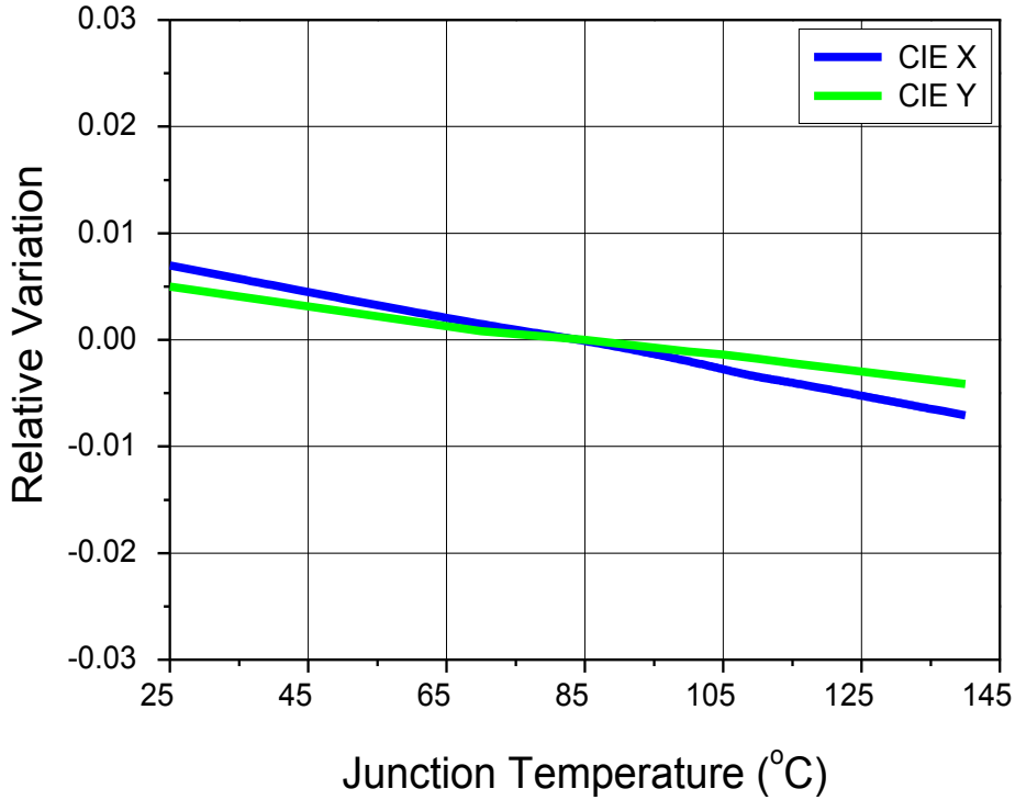
Fig 16. Junction Temperature vs. CIE x,y Shift, I_f=0.24A (CRI90, Neutral White)
