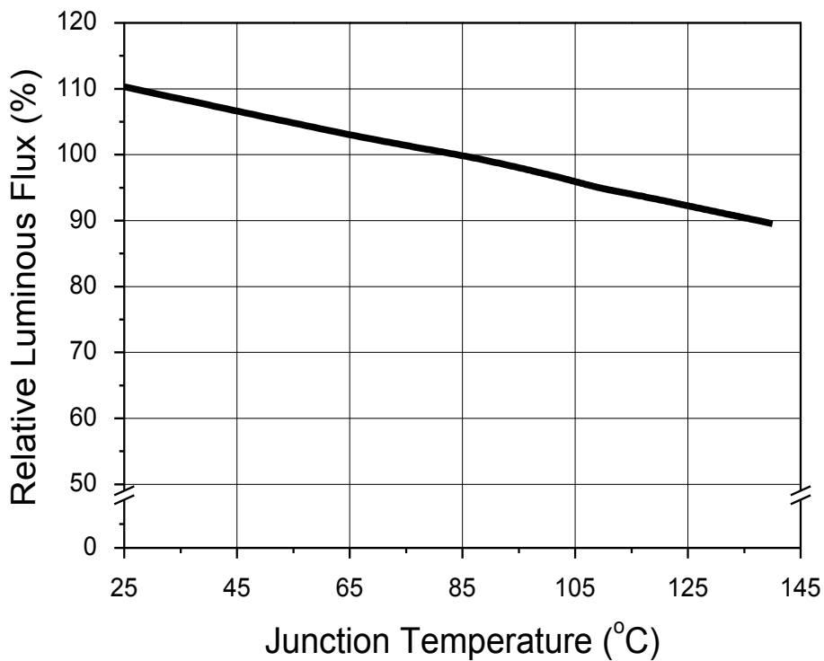
Fig 12. Junction Temperature vs. Relative Luminous Flux, I_F=0.24A
