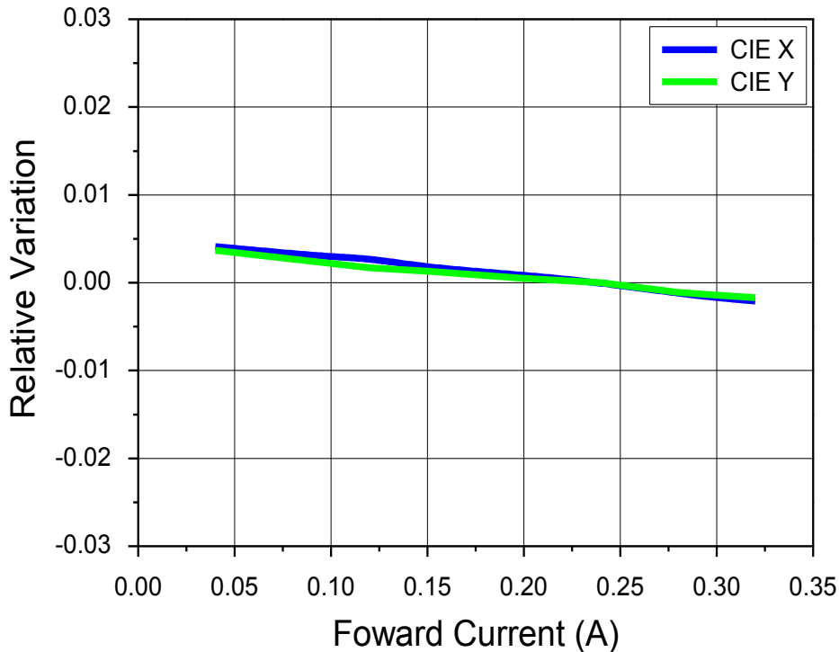
Fig 9. Forward Current vs. CIE x,y Shift (CRI90, Neutral White)
