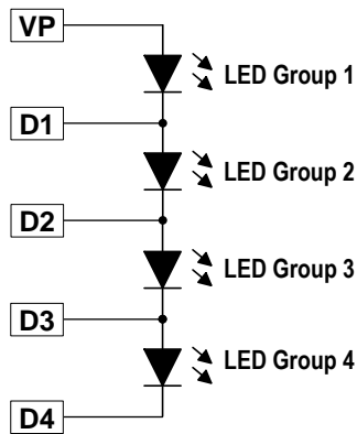
< Inner Circuit Diagram >
