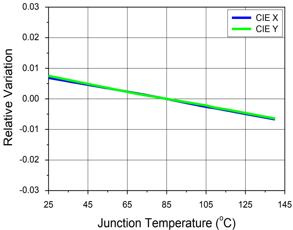
Fig 14. Junction Temperature vs. CIE x,y Shift, I_f=0.24A (CRI80, Neutral White)
