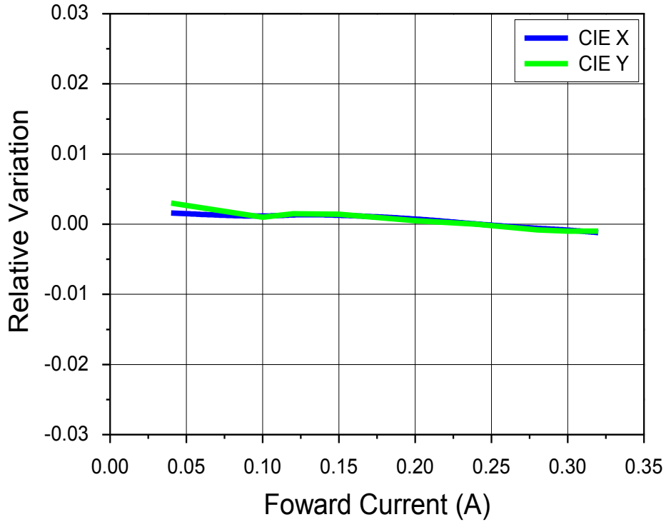
Fig 10. Forward Current vs. CIE x,y Shift (CRI90, Warm White)
