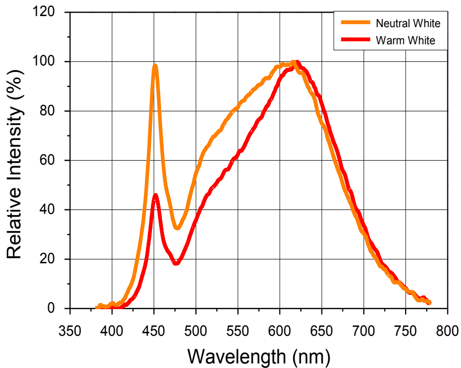
Fig 2. Color Spectrum, CRI90
