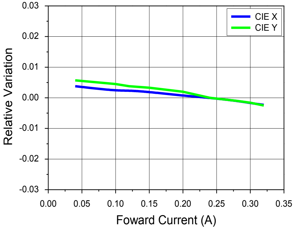
Fig 6. Forward Current vs. CIE x,y Shift (CRI80, Cool White)
