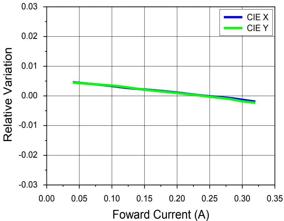
Fig 7. Forward Current vs. CIE x,y Shift (CRI80, Neutral White)
