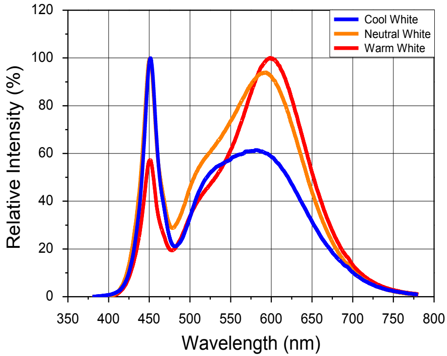
Fig 1. Color Spectrum, CRI80
