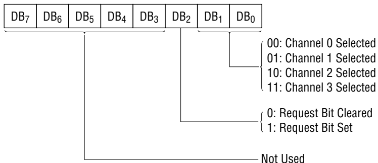
Figure 5 Request Register
