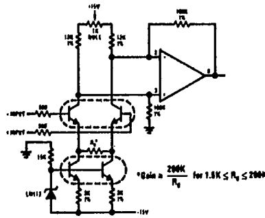
Instrumentation Amplifier
