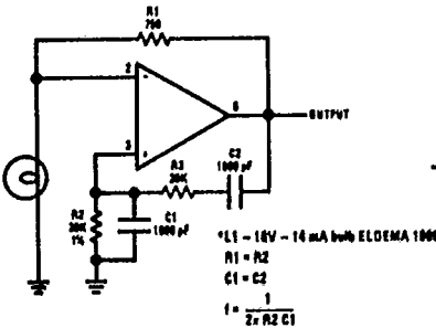
Wein Bridge Sine Wave Oscillator
