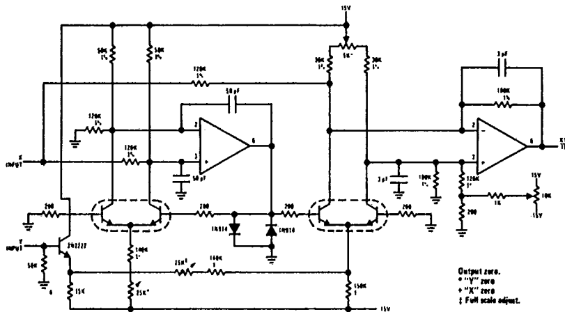
Four Quadrant Multiplier
