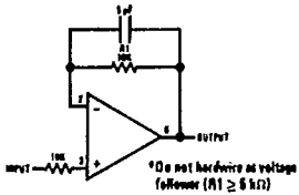
Fast Voltage Follower *
