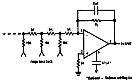
D/A Converter Using Ladder Network
