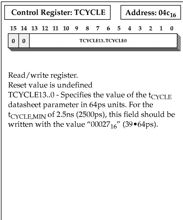
Figure 42: TCYCLE Register
