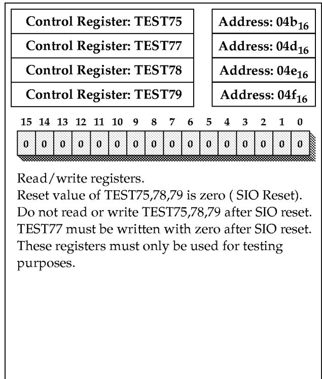
Figure 43: TEST Registers
