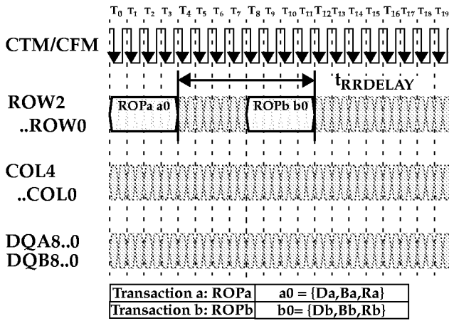
Figure 6: ROW-to-ROW Packet Interaction- Timing
