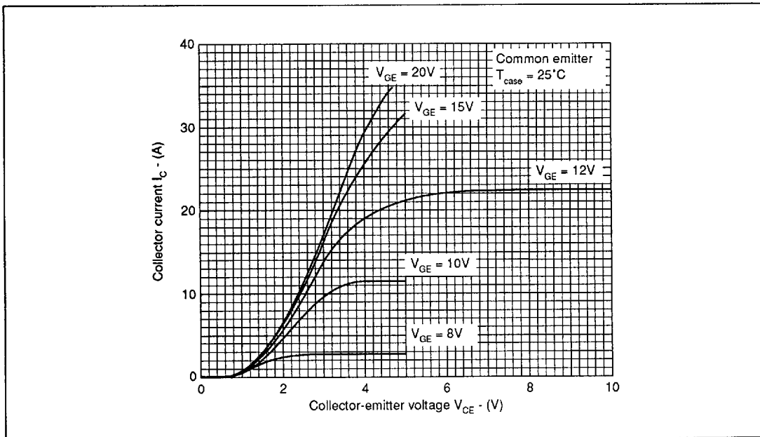
Fig.6 Typical output characteristics
