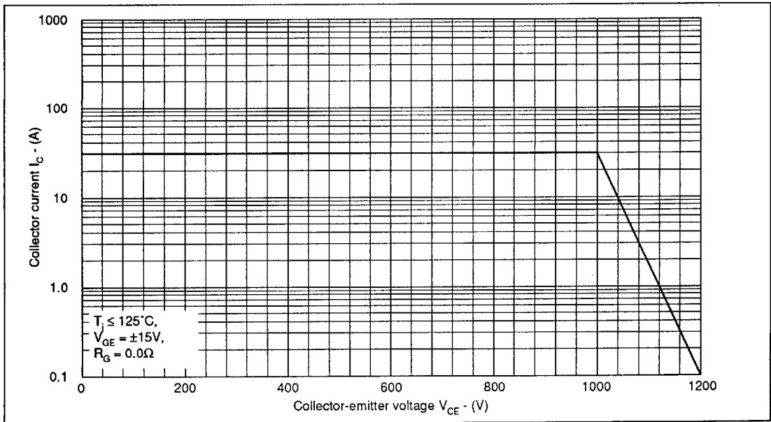
Fig.13 Reverse bias safe operating area
