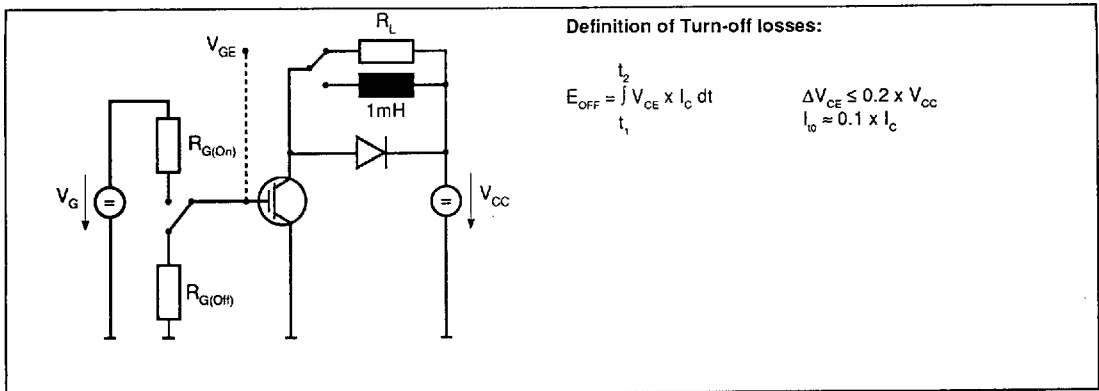
Fig.3 Test circuit
