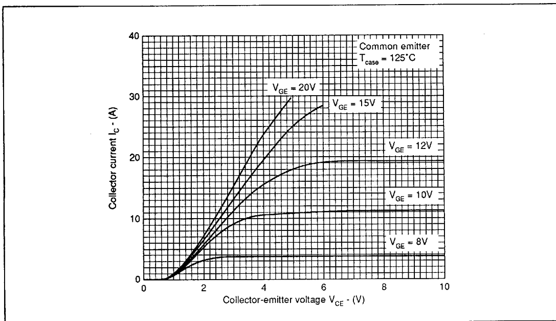
Fig.7 Typical output characteristics
