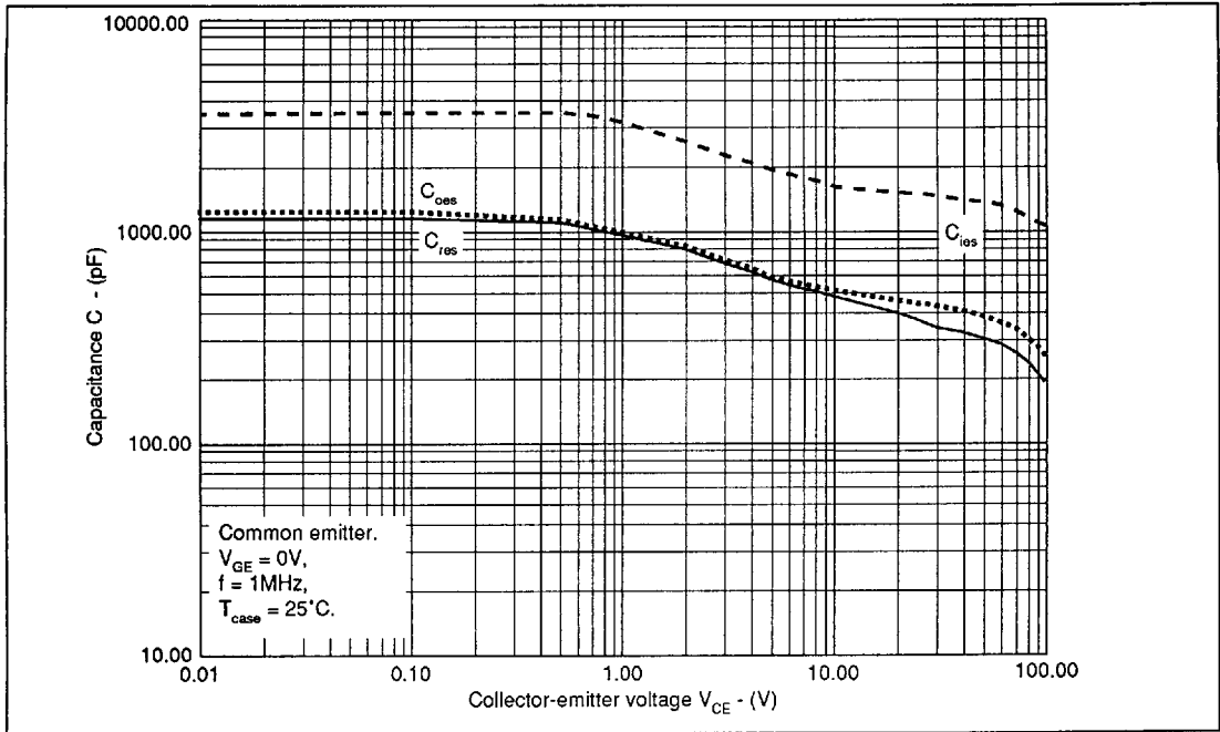
Fig.12 Typical capacitance
