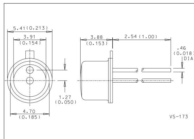
Modified TO-18 Package.
