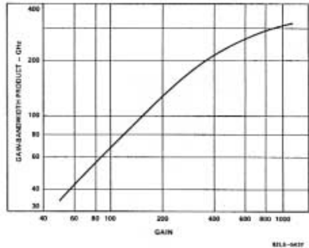
Figure 5. Typical Gain-Bandwidth Product vs. Gain
