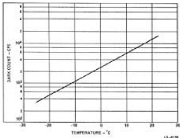
Figure 11. Typical Dark Count vs. Temperature at 5% Photon (830 nm) Detection Efficiency
