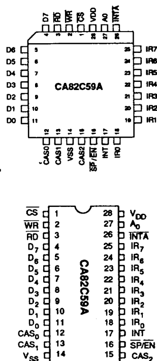
Figure 2 : PLCC and DIP PIN CONFIGURATIONS
