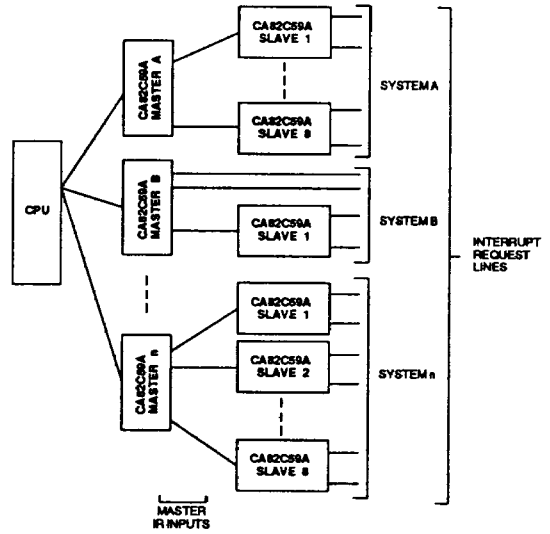
Figure 24 : CA82C59A IN STANDARD SYSTEM CONFIGURATION
