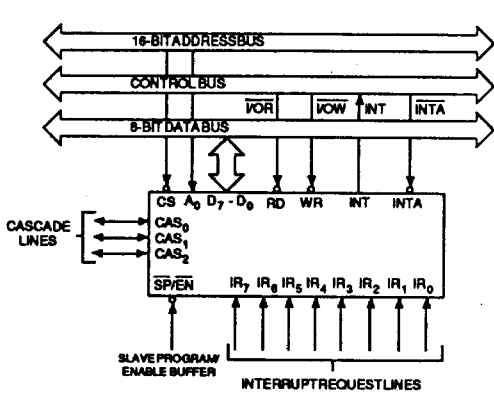
Figure 24 : CA82C59A IN STANDARD SYSTEM CONFIGURATION
