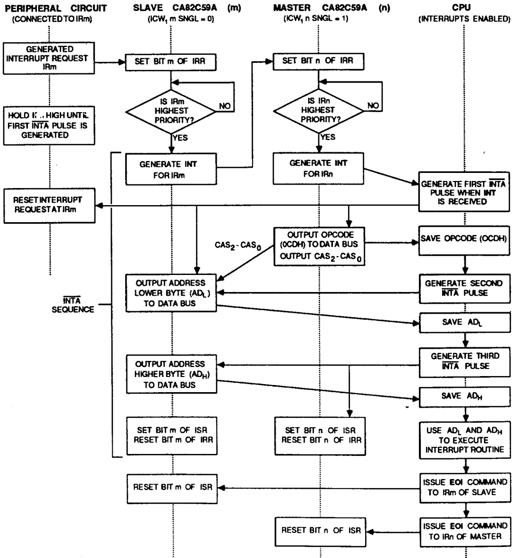
Figure 8 : CALL MODE OPERATION (Cascaded CA82C59A Systems)
