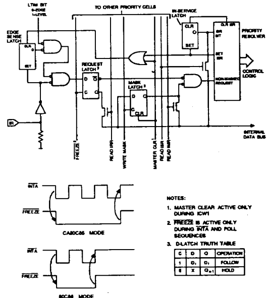
Figure 23 : PRIORITY CELL STRUCTURE
