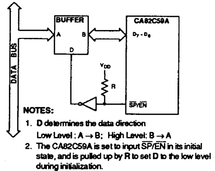
Figure 15 : BUFFER MODE
