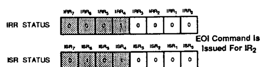
Figure 18 : FULLY NESTED MODE
