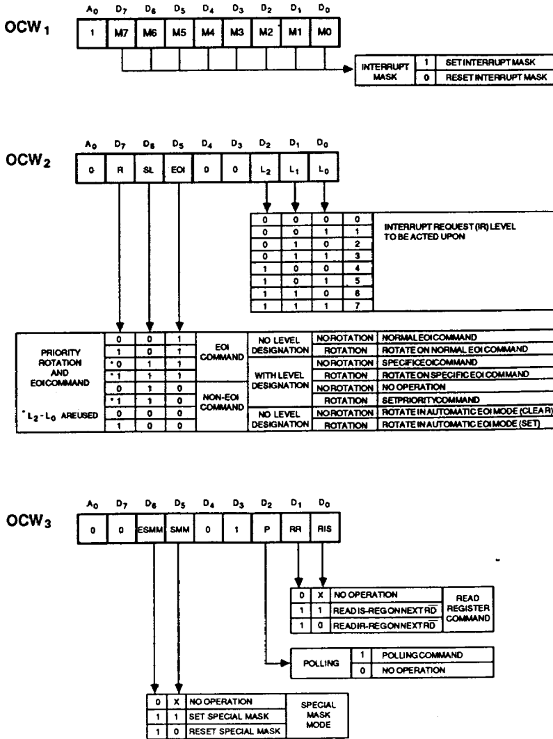
Figure 14 : OPERATIONAL COMMAND WORD FORMAT
