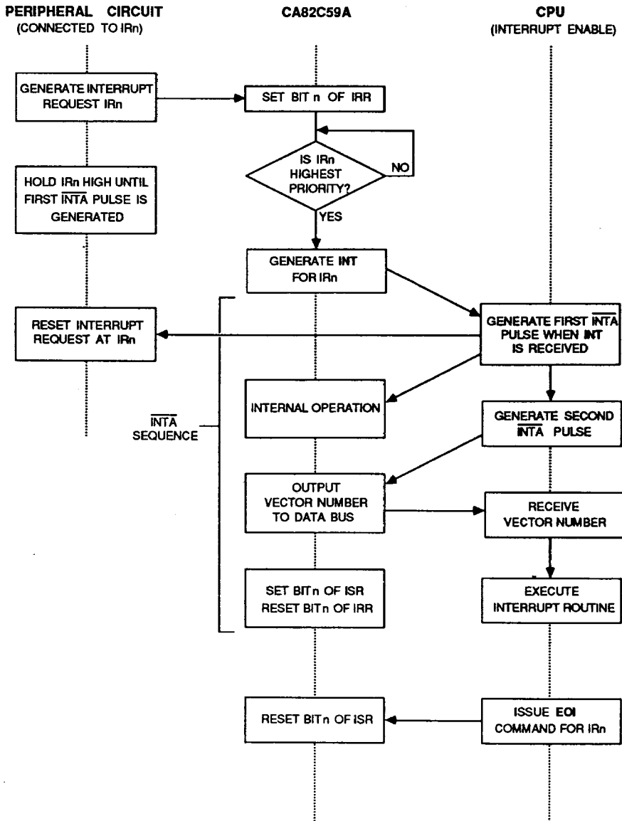
Figure 9 : VECTOR MODE OPERATION (Single CA82C59A Systems)
