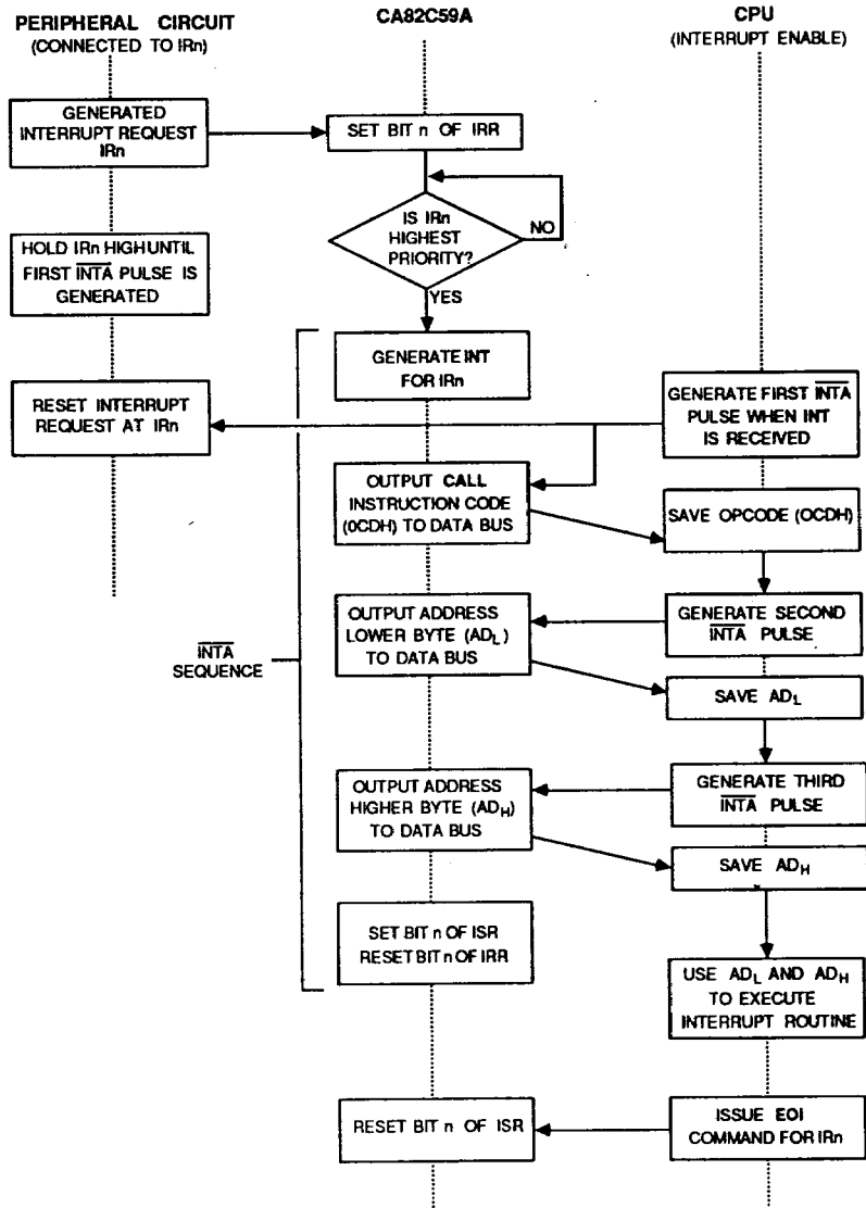
Figure 6 : CALL MODE OPERATION (Single CA82C59A Systems)
