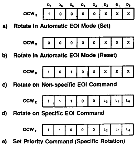
Figure 21 : ROTATION COMMANDS
