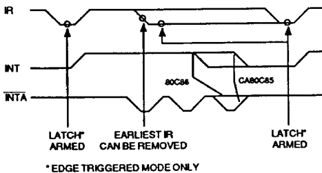
Figure 22 : TRIGGER MODE TIMING
