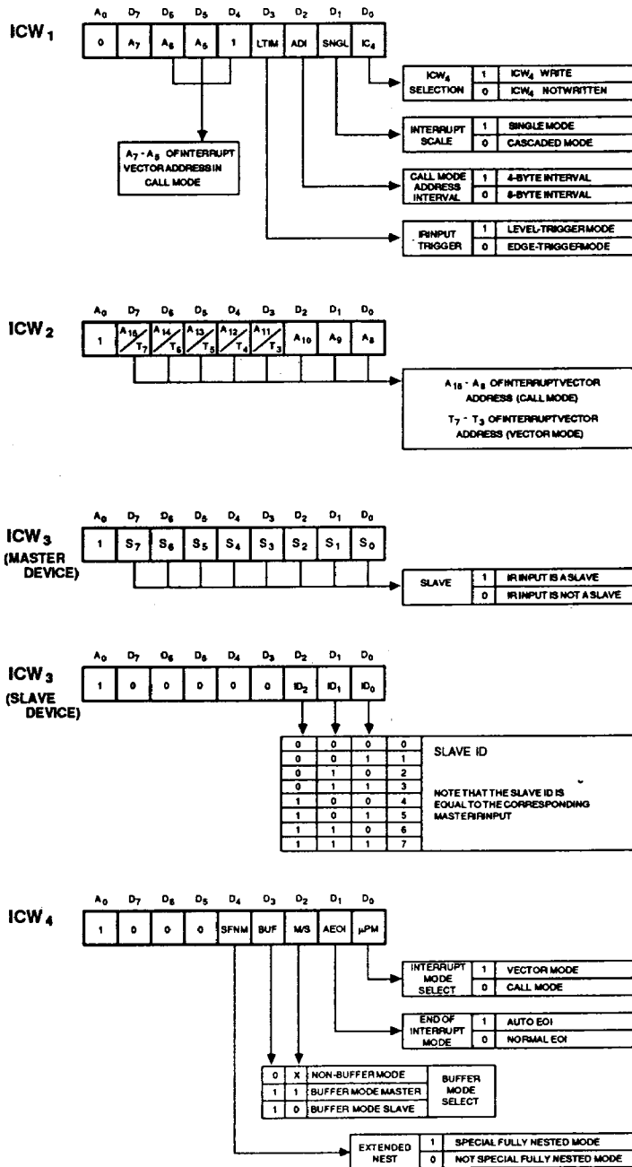
Figure 13 : INITIALIZATION COMMAND WORD FORMAT
