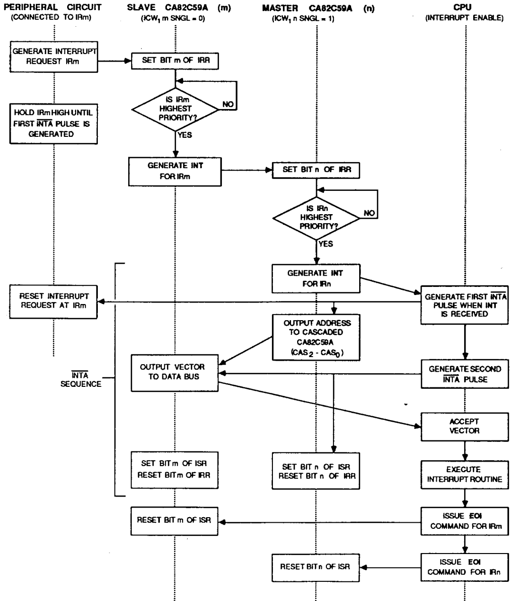
Figure 11 : VECTOR MODE OPERATION (Cascaded CA82C59A Systems)
