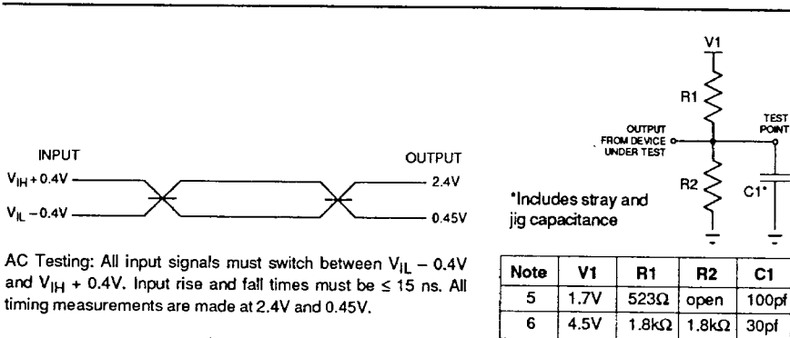
Figure 4 : AC TESTING I/O WAVEFORMS
