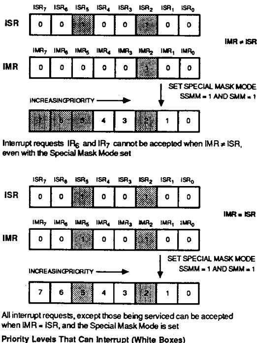
Figure 17 : SPECIAL MASK MODE
