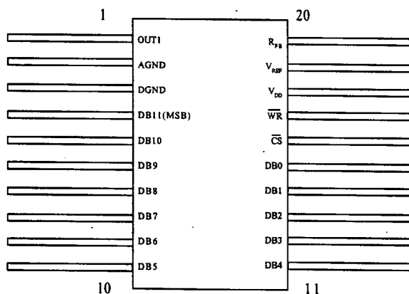
PIN CONFIGURATION
