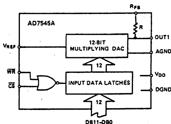
7545ARP Functional Block Diagram
