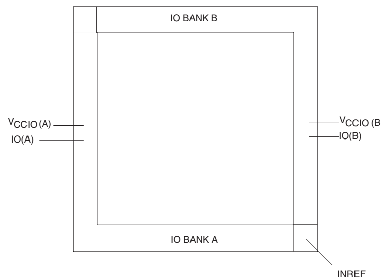
Figure 47: QL5822 I/O Banks with Relevant Pins
