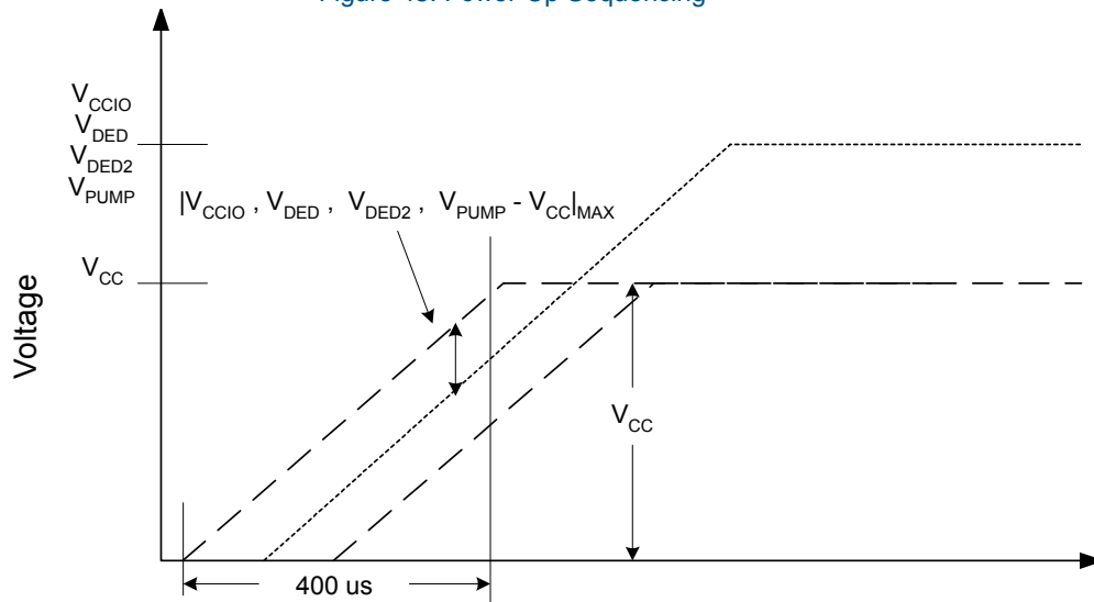
Figure 45: Power-Up Sequencing
