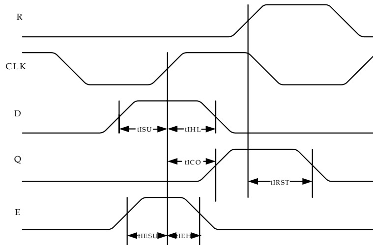
Figure 42: QL58x2 Device Family Input Register Cell Timing
