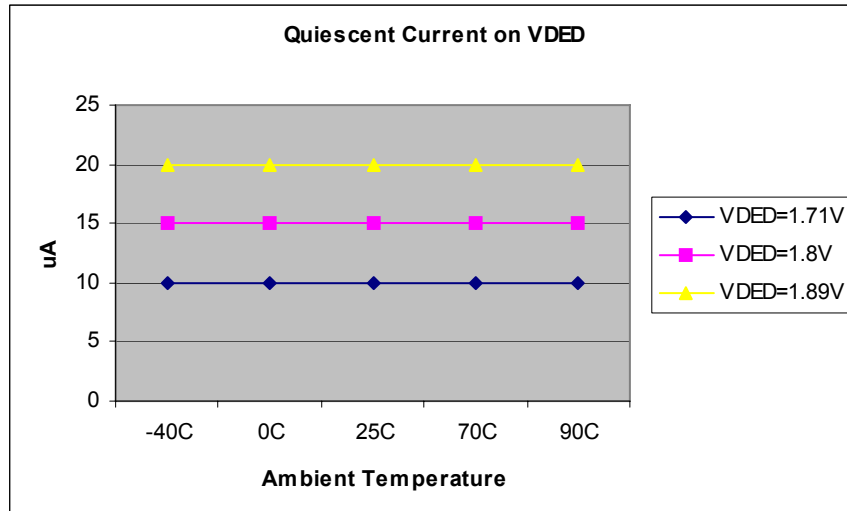
Figure 28: Quiescent Current for QL5842 at V_{DED} = 1.8 V
