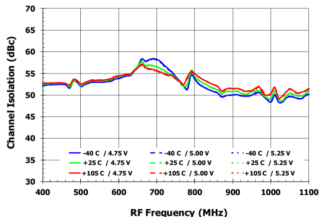
Channel Isolation vs. T_{case} & V_{cc} [ ISO_{A-B} ]
