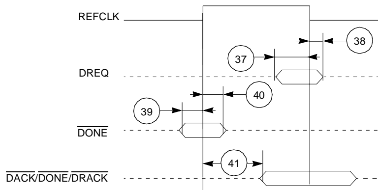
Figure 2-4. DMA Signals
