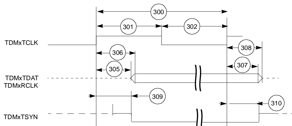
Figure 2-10. TDM Output Signals
