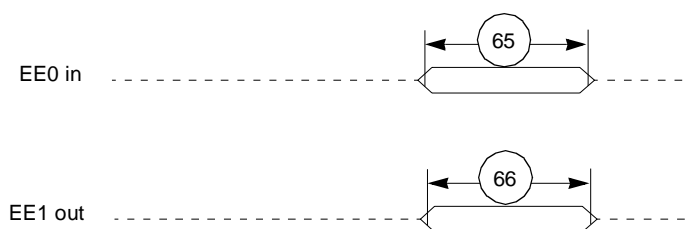
Figure 2-15. EE Pins Timing
