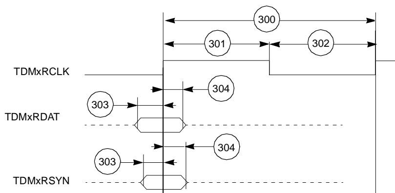
Figure 2-9. TDM Inputs Signals
