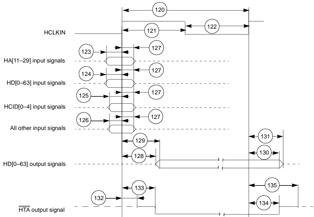
Figure 2-8. DSI Synchronous Mode Signals Timing Diagram
