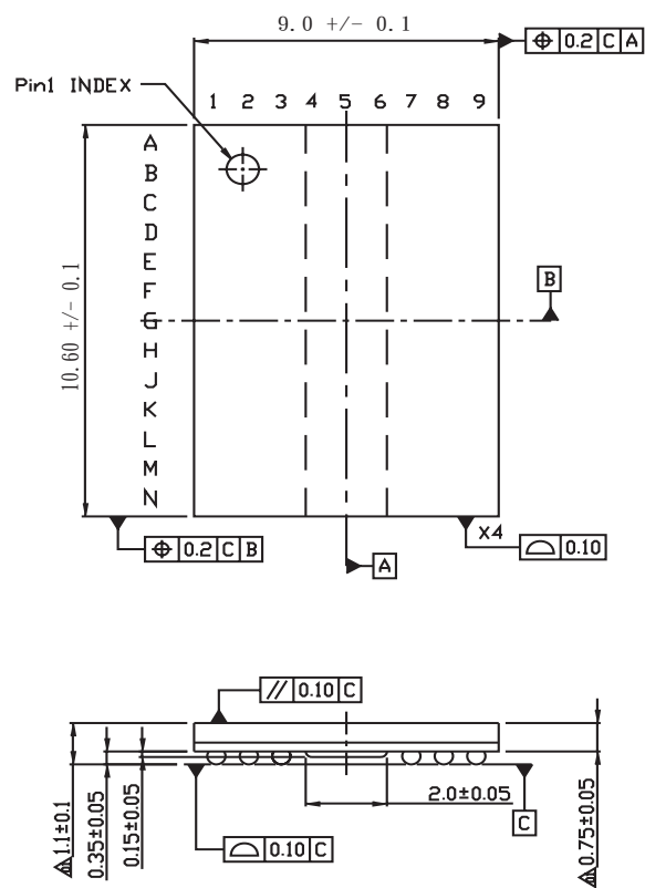
Package Diagram (x8) 78-Ball Fine Pitch Ball Grid Array Outline
