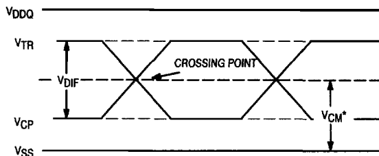
Figure 3. Differential Inputs/Common Mode Input Voltage
