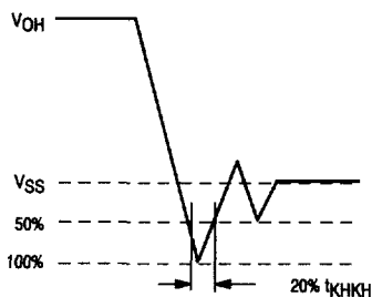
Figure 2. Undershoot Voltage
