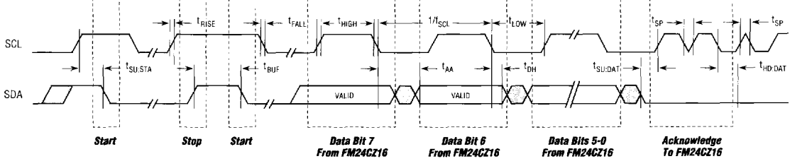
Figure 3. Bus Timing
