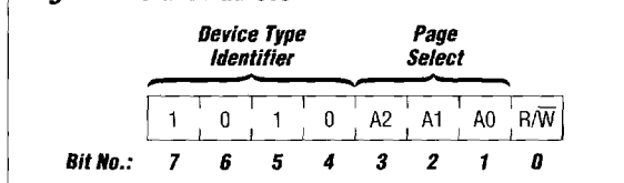
Figure 4. Slave Address
