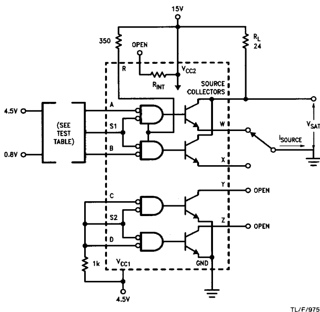
FIGURE 3. V_{IL} and Source V_{SAT}
