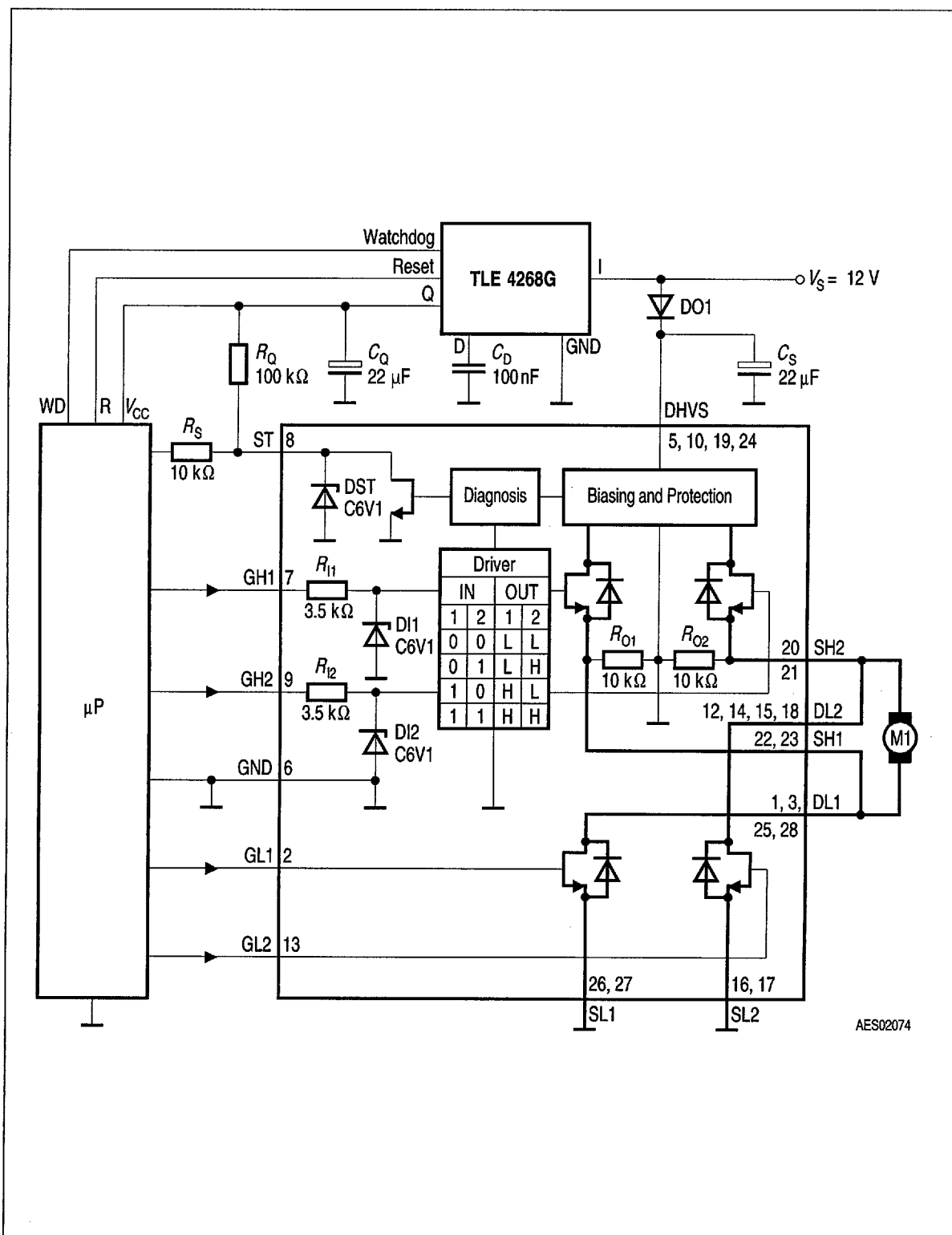
Figure 4 Application Circuit
