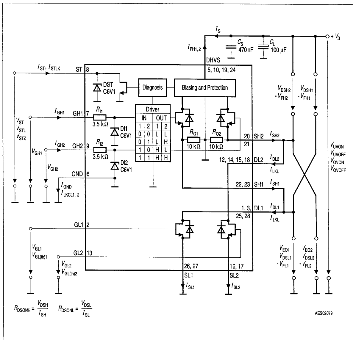
Figure 3 Test Circuit
