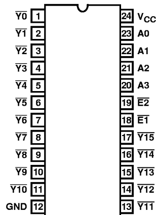
CD74HC154, CD74HCT154 (PDIP, SOIC) TOP VIEW
