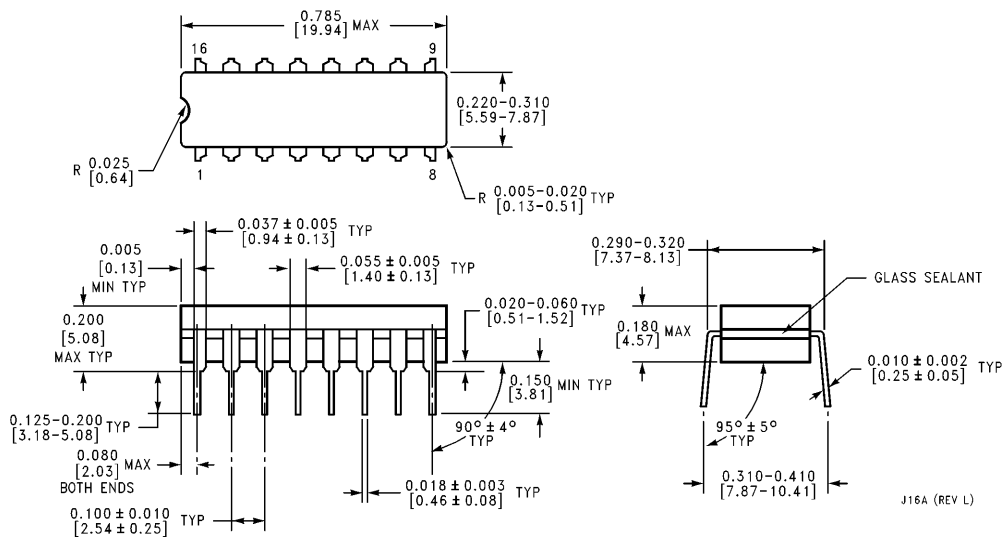
16-Lead Ceramic Dual-In-Line Package (J) Order Number DM54109J NS Package Number J16A
