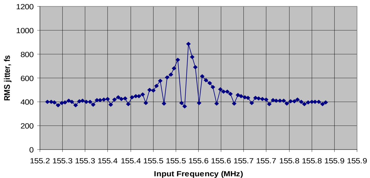
Figure 87. \pm 2000 ppm, 50 ppm Steps
