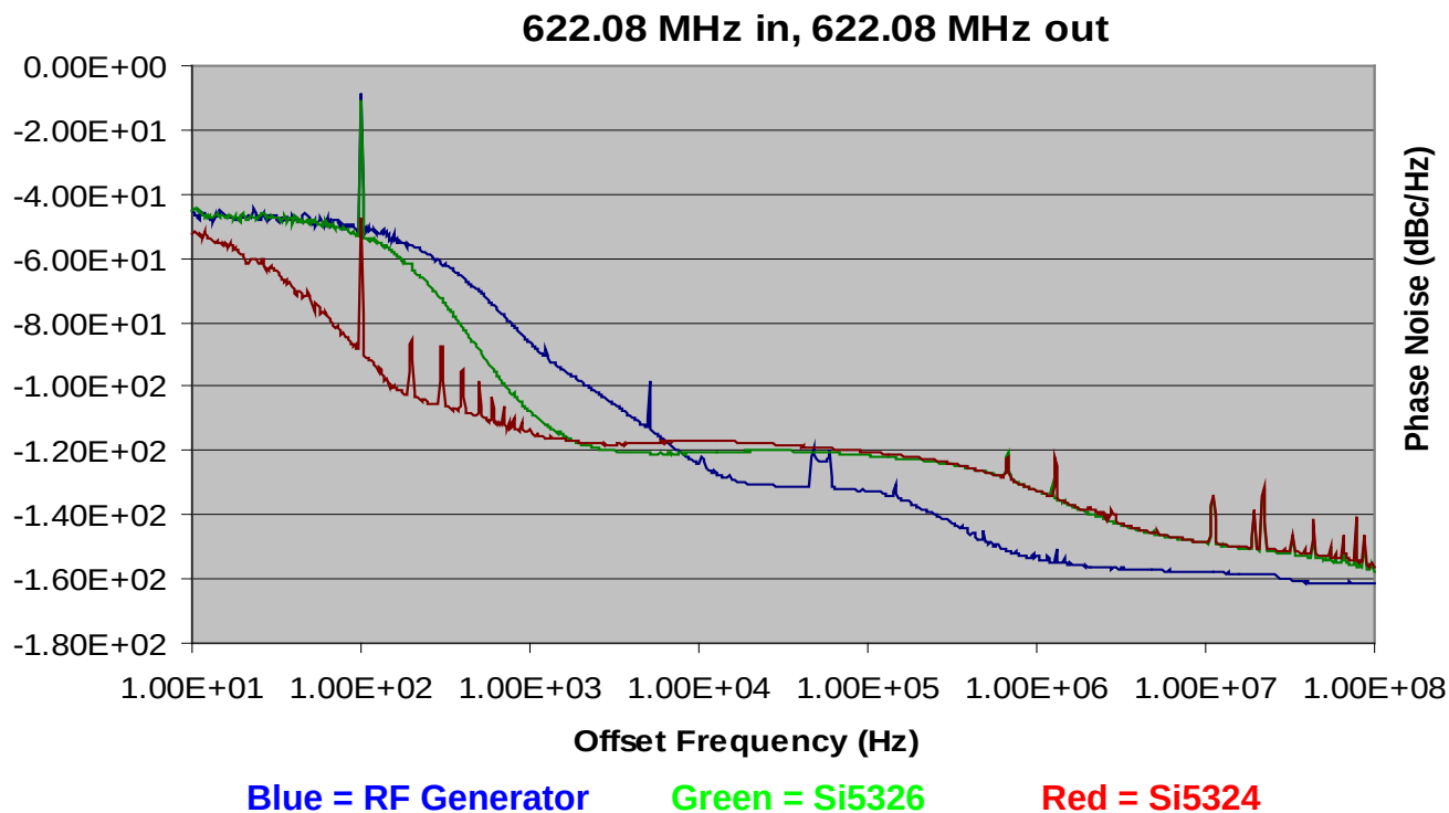
Figure 90. RF Generator, Si5326, Si5324 (100 Hz Jitter)
