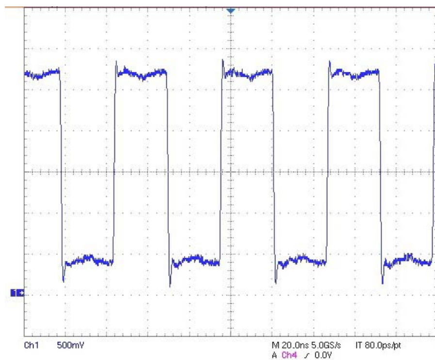
Figure 46. sfout_2, CMOS
