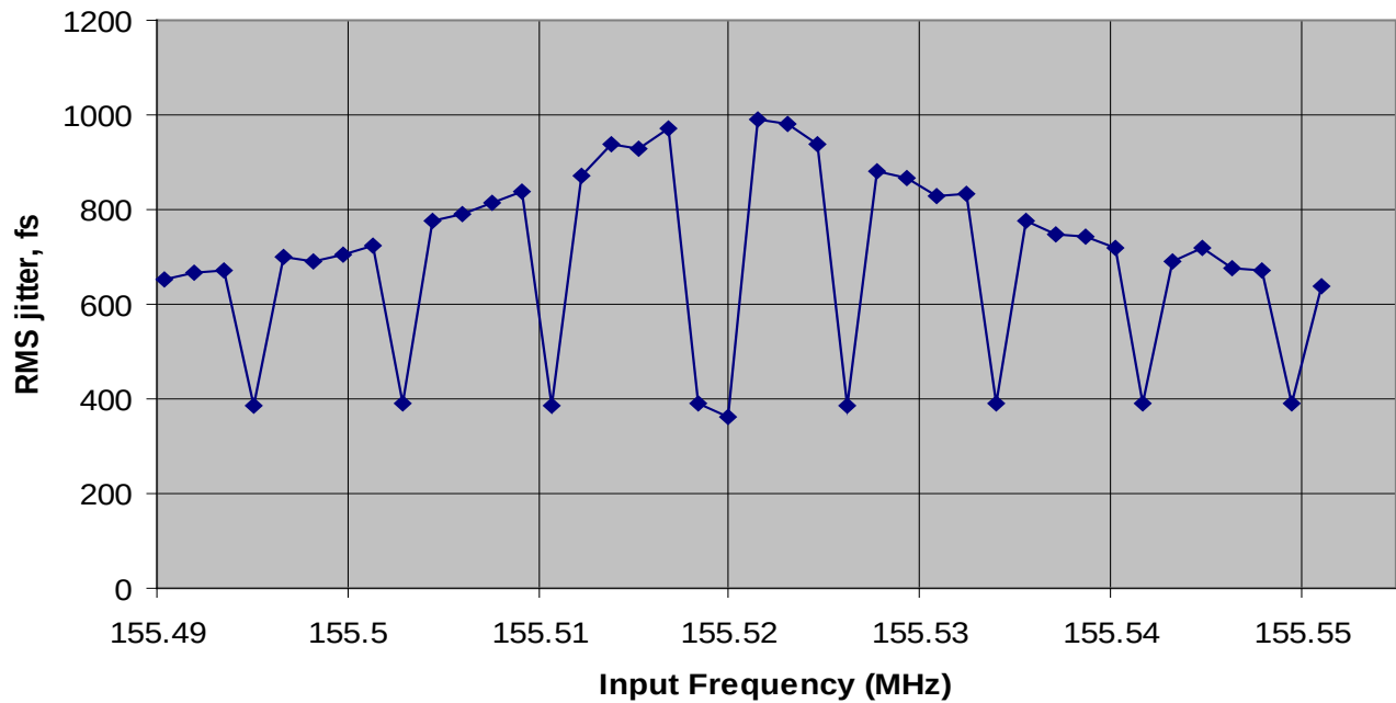
Figure 86. \pm 200 ppm, 10 ppm Steps
