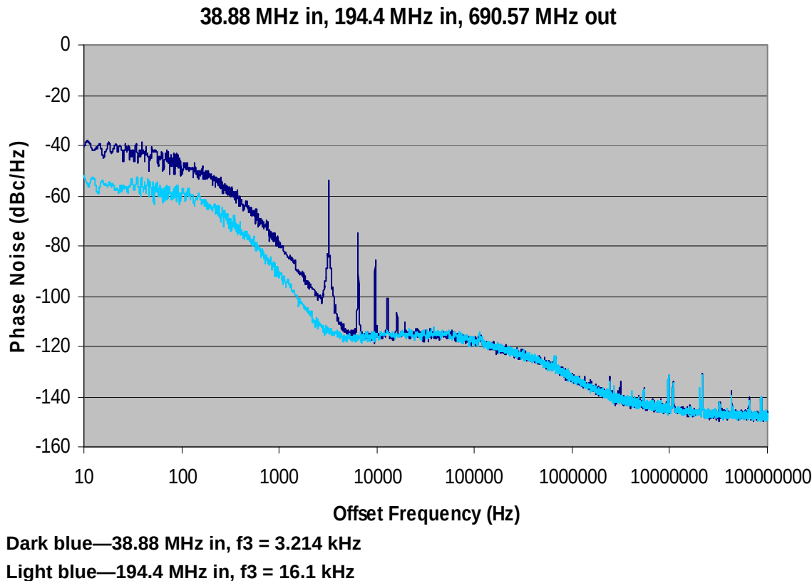
Figure 61. Jitter vs. f3 with FPGA
