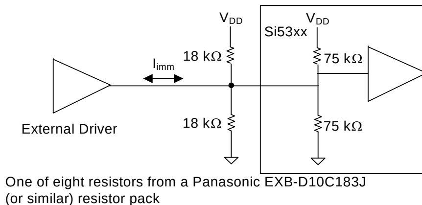
Figure 56. Three Level Input Pins
