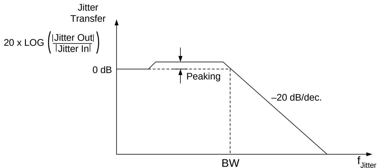
Figure 22. PLL Jitter Transfer Mask/Template
