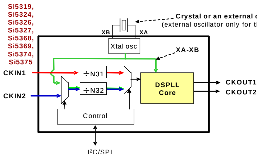
Figure 29. Free Run Mode Block Diagram
