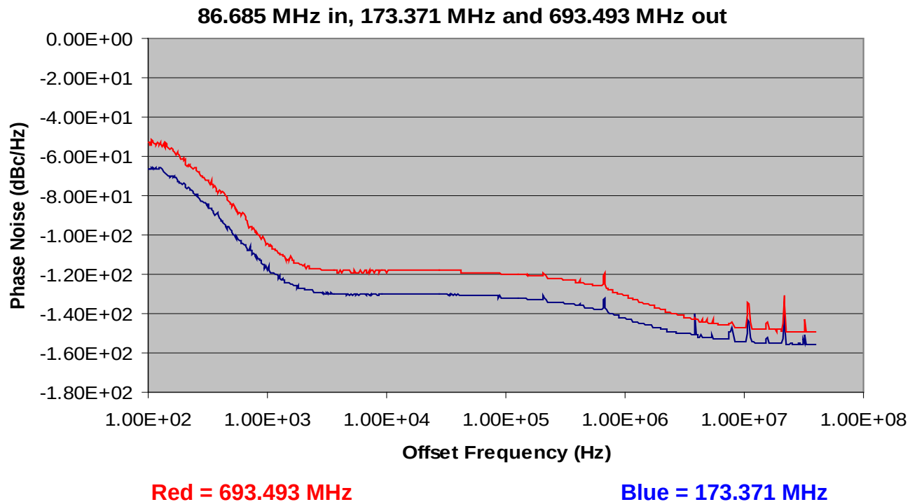
Figure 77. 86.685 MHz In; 173.371 MHz and 693.493 MHz Out
