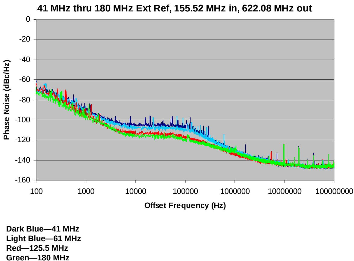
Figure 64. Jitter vs. Reference Frequency (2 of 2)
