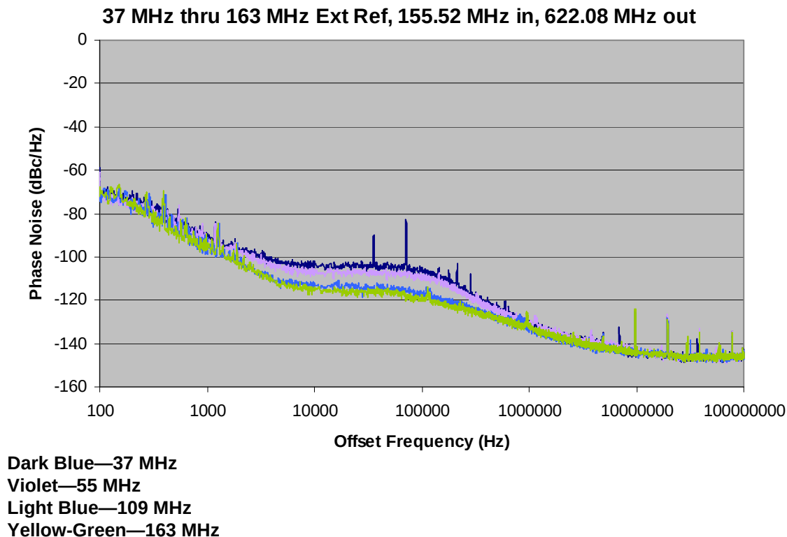
Figure 63. Jitter vs. Reference Frequency (1 of 2)
