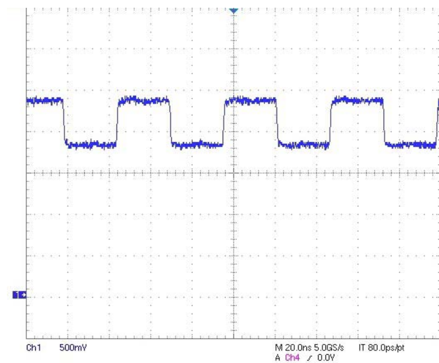
Figure 47. sfout_3, lowSwingLVDS
