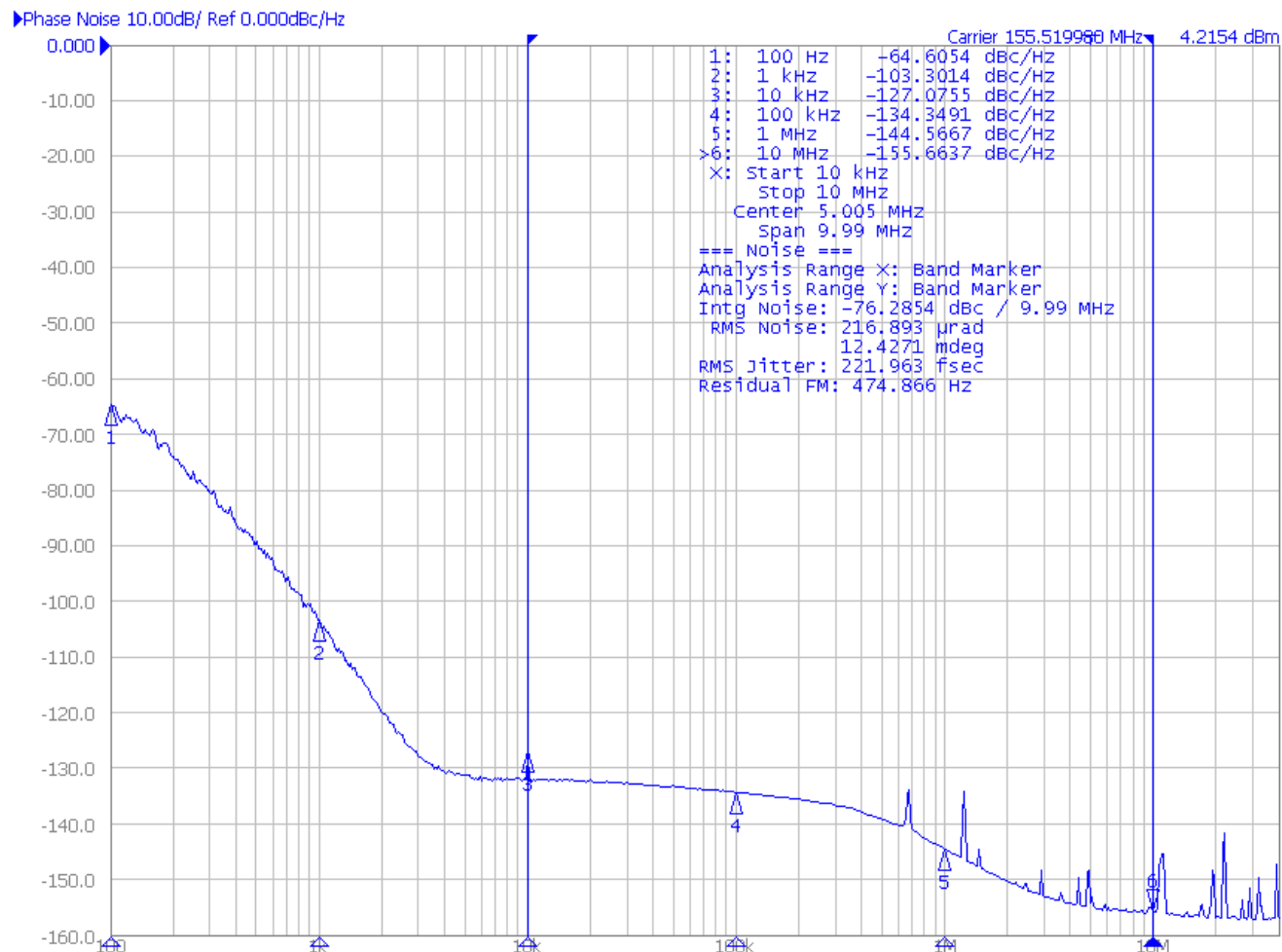
Figure 73. 156.25 MHz In; 155.52 MHz Out
