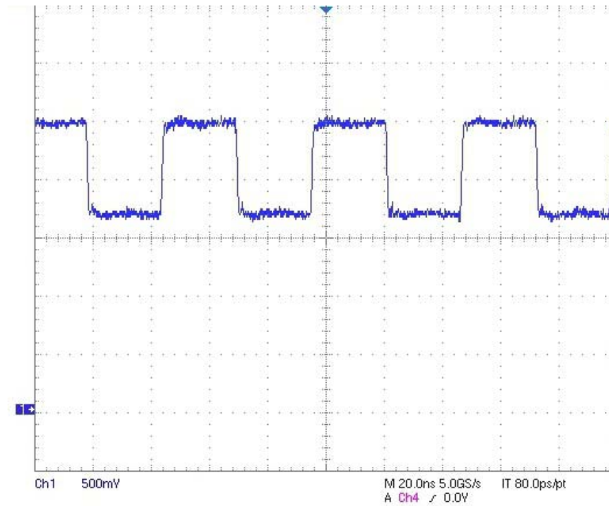
Figure 48. sfout_5, LVPECL
