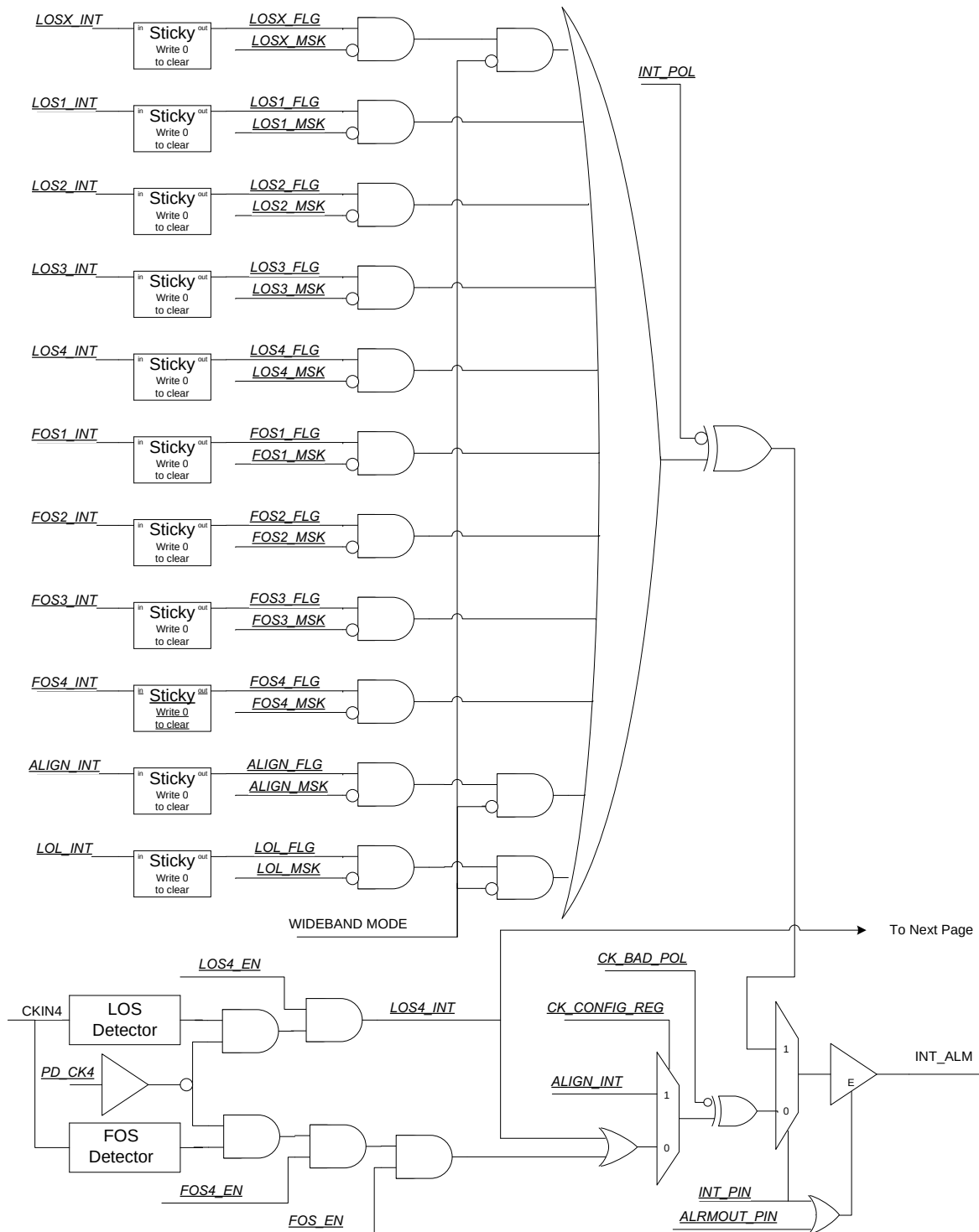
Figure 83. Si5368 and Si5369 Alarm Diagram (1 of 2)
