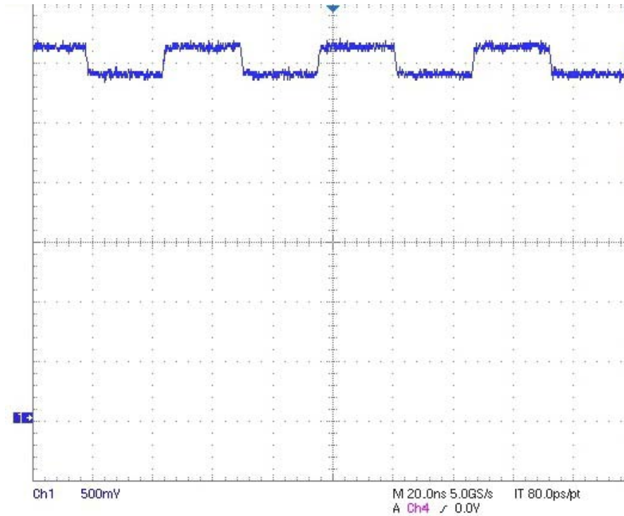
Figure 49. sfout_6, CML
