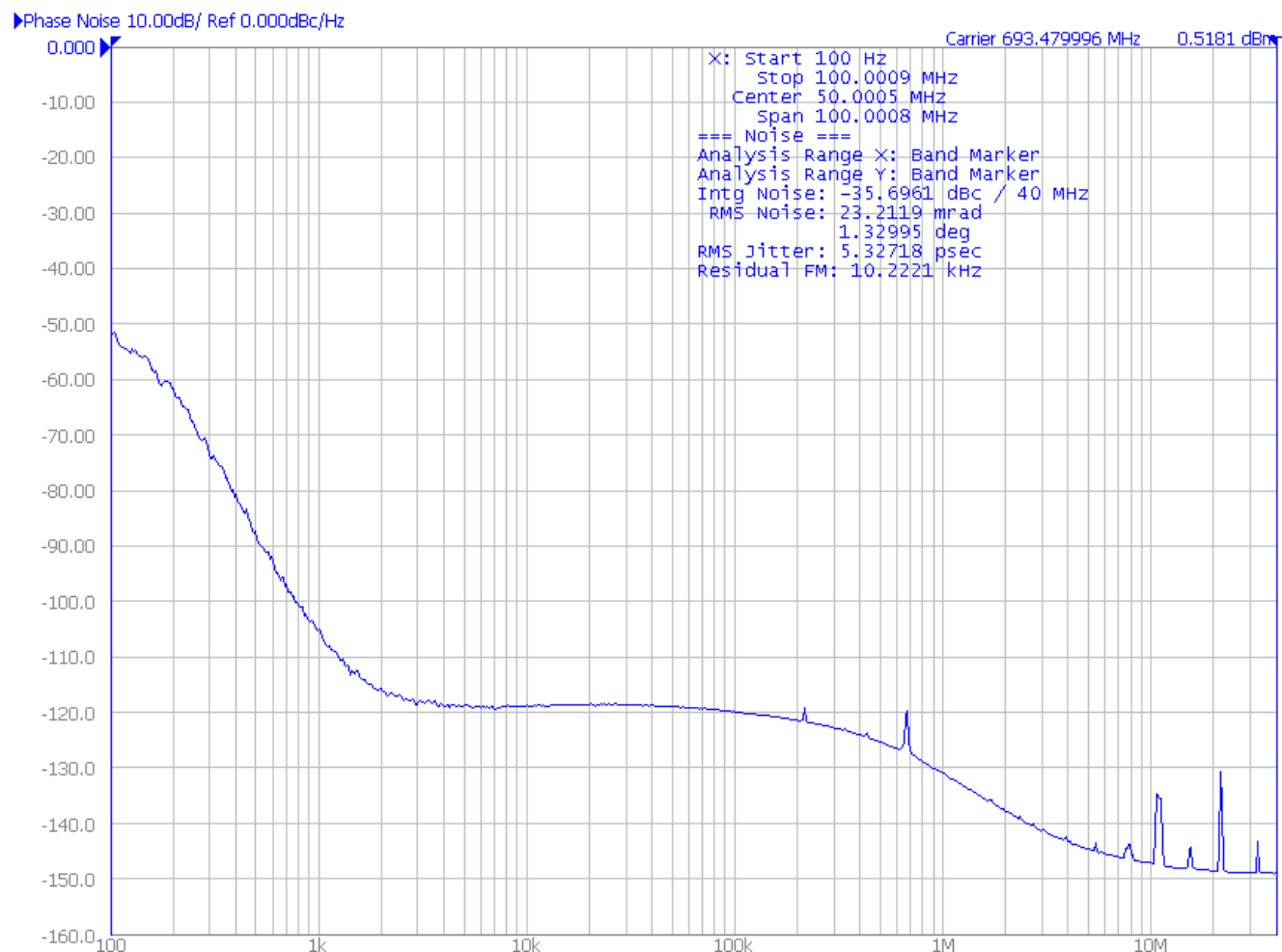
Figure 79. 86.685 MHz In; 693.493 MHz Out
