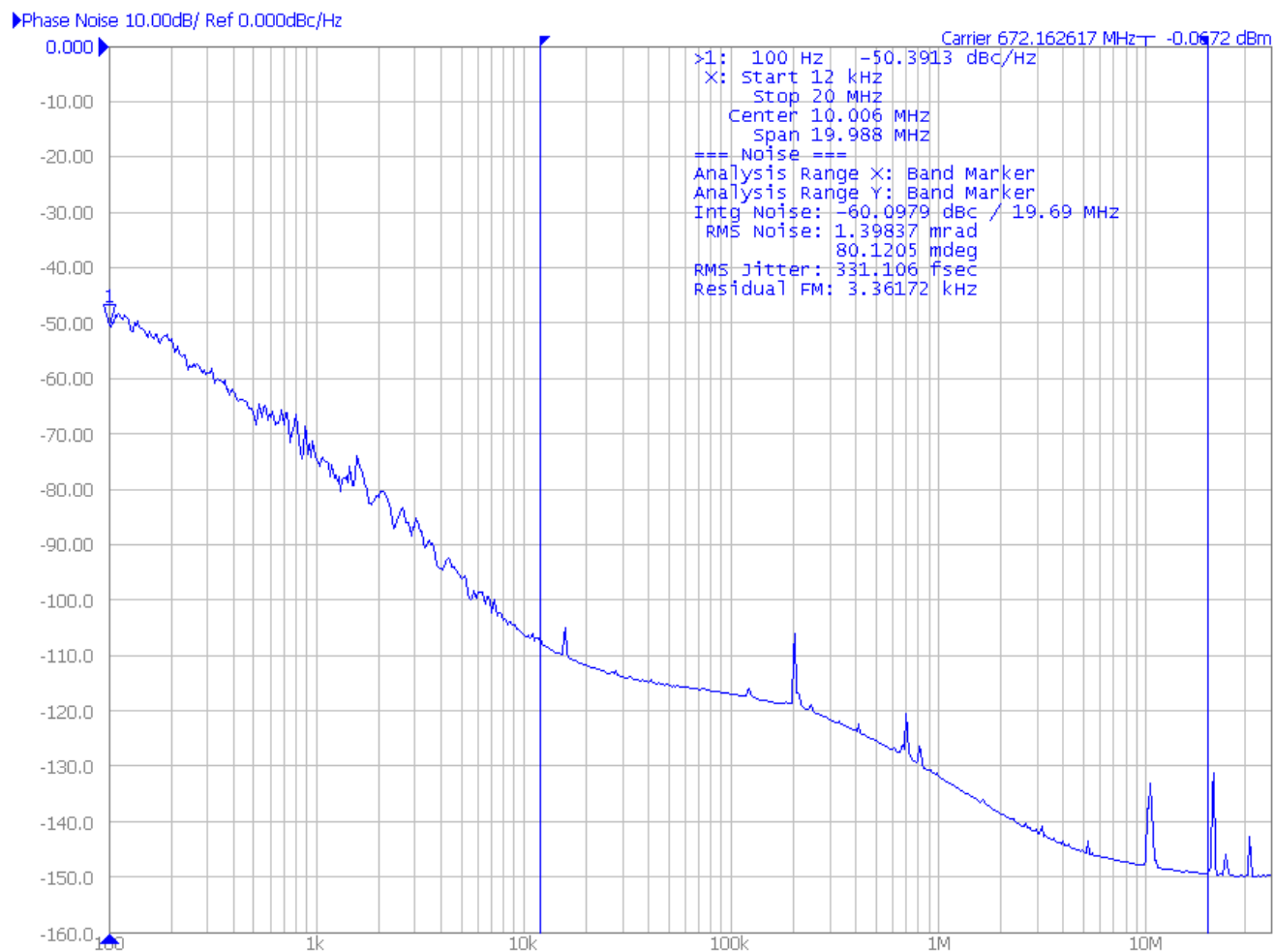
Figure 71. 622.08 MHz In; 672.16 MHz Out; Loop BW = 6.9 kHz
