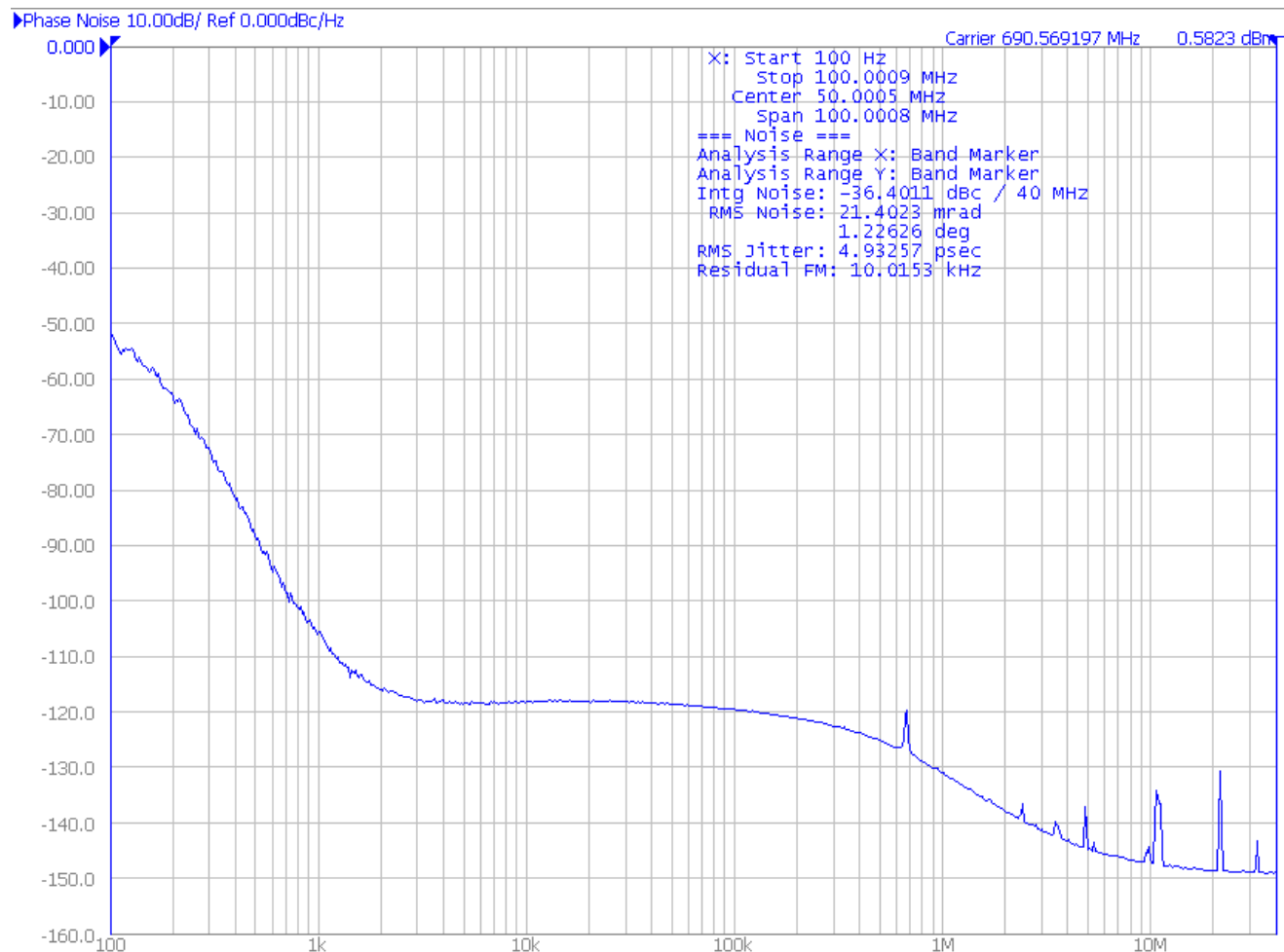
Figure 75. 78.125 MHz In; 690.569 MHz Out
