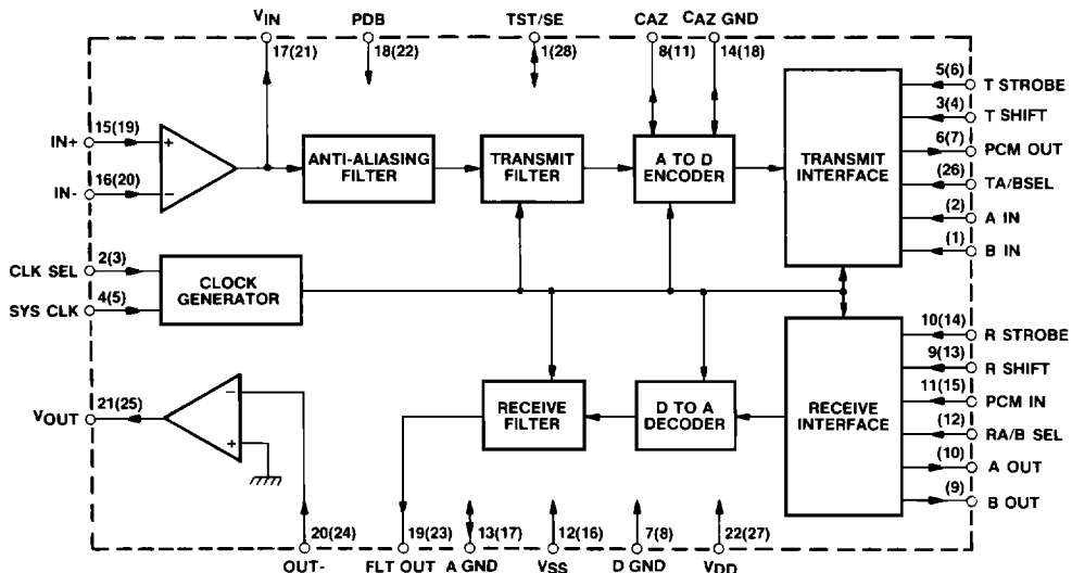
Fig.2 Functional block diagram (pin numbers for the MV3507A are in brackets)
