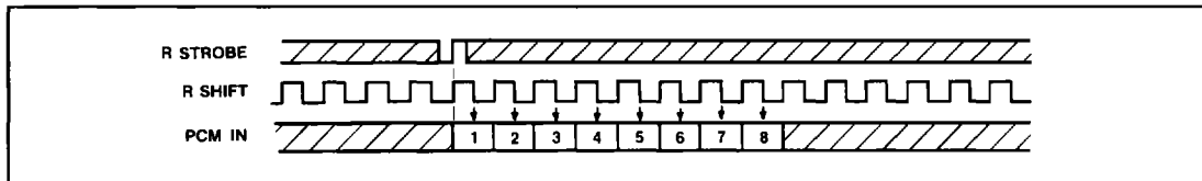
Fig.6 Receive alignment
