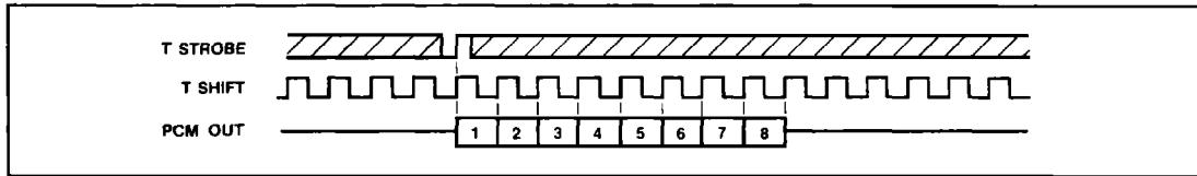
Fig.4 Transmit alignment
