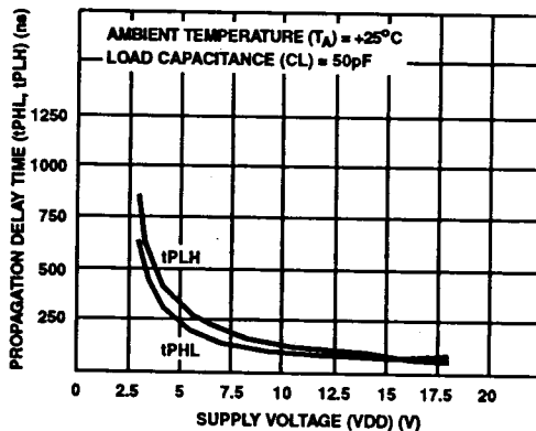
FIGURE 7. TYPICAL DATA PROPAGATION DELAY TIME vs SUPPLY VOLTAGE
