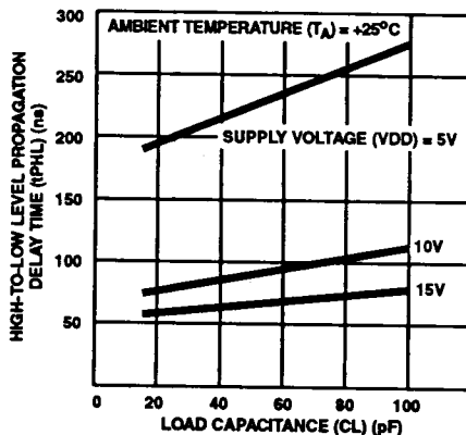
FIGURE 5. TYPICAL DATA HIGH-TO-LOW LEVEL PROPAGATION DELAY TIME vs LOAD CAPACITANCE
