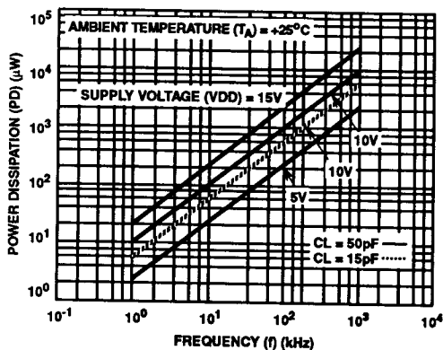
FIGURE 4. TYPICAL POWER DISSIPATION vs FREQUENCY
