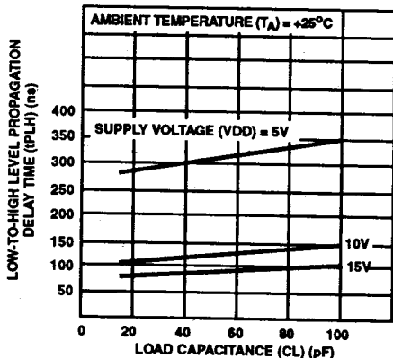
FIGURE 6. TYPICAL DATA LOW-TO-HIGH LEVEL PROPAGATION DELAY TIME vs LOAD CAPACITANCE
