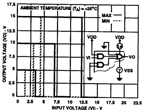
FIGURE 3. MINIMUM AND MAXIMUM VOLTAGE TRANSFER CHARACTERISTICS
