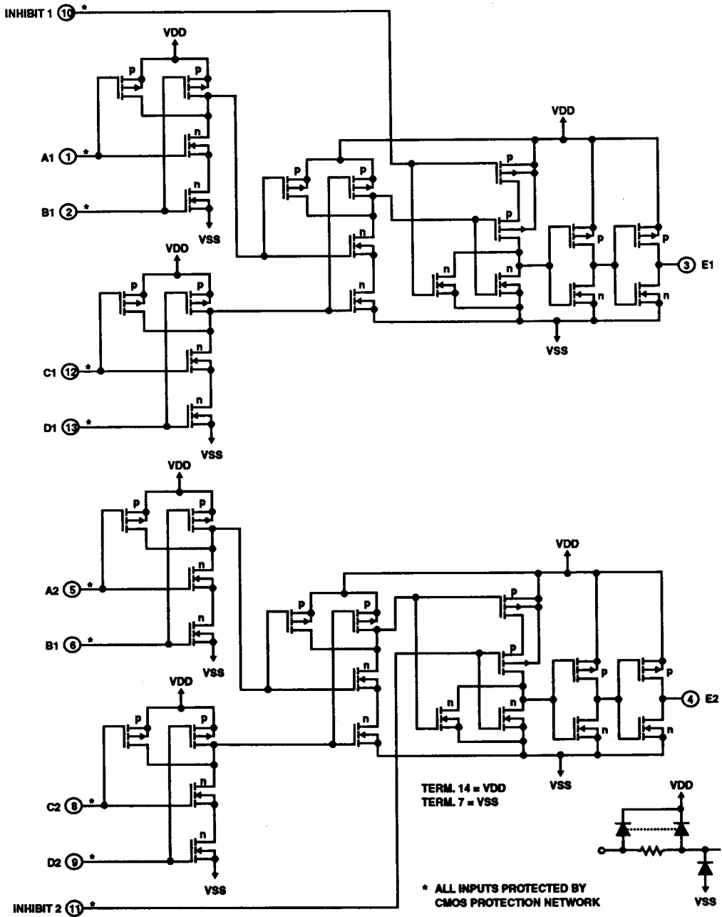
FIGURE 1. CD4085B SCHEMATIC DIAGRAM
