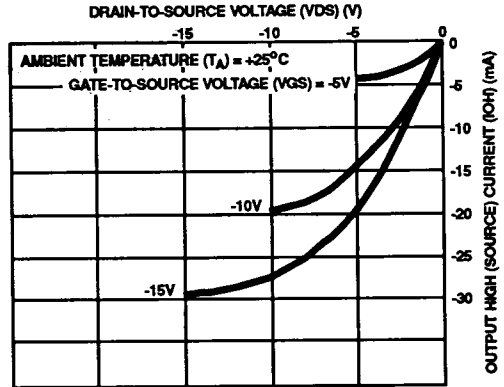
FIGURE 11. TYPICAL OUTPUT HIGH (SOURCE) CURRENT CHARACTERISTICS
