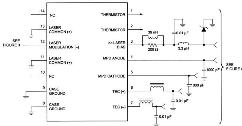
Figure 2. 1754W Circuit Schematic
