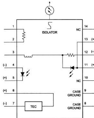
Figure 1. 1754W Laser Schematic
