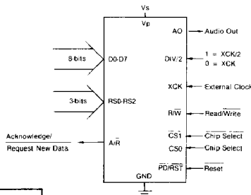
Signal Diagram
