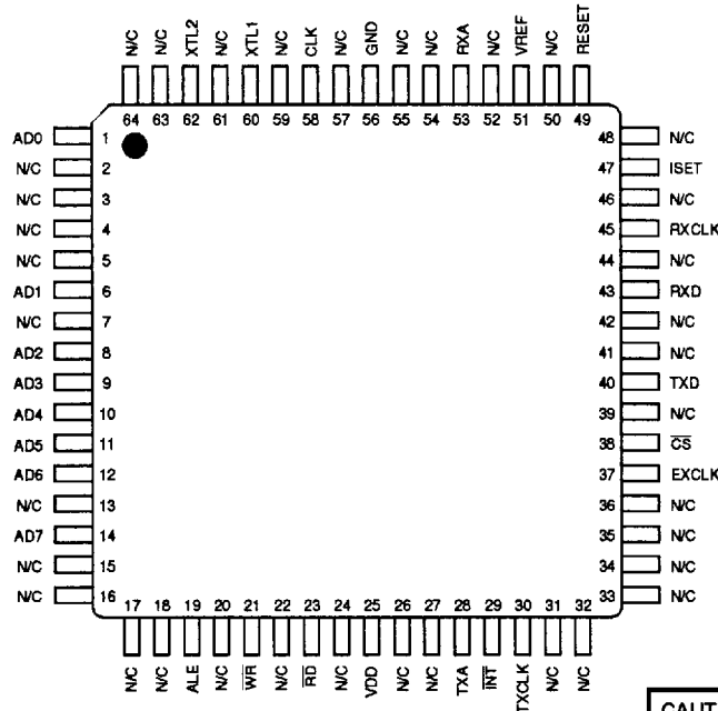
64-Lead TQFP
