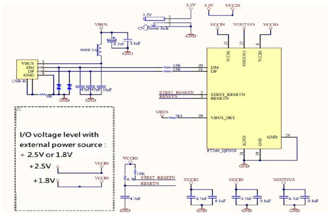
Figure 7-5 Self-Powered Configuration with +1.8V/+2.5V I/O voltage Level
