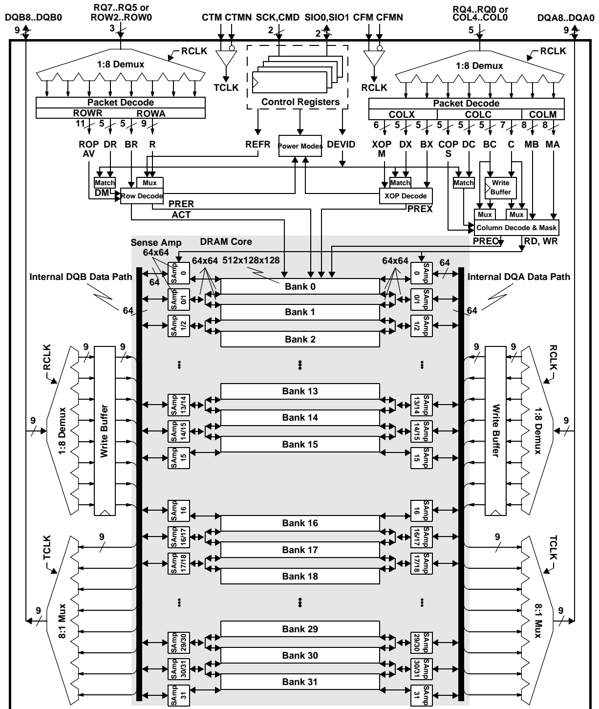
Figure 2: 256Mbit (512Kx16x32s) RDRAM Device Block Diagram
